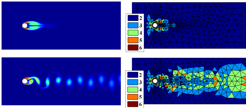
Figure 17: Von Kármán street past a cylinder at Re=100 : vorticity pattern (left) and degree map (right) at a time step, t = 14 , before (top) and, t = 750 , after (bottom) the initiation of the shedding .
