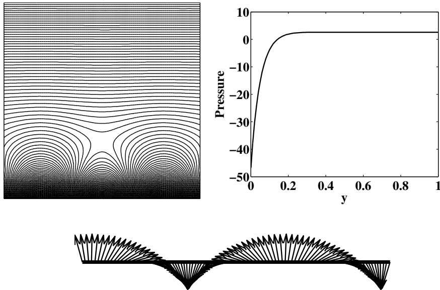
Figure 3: Wang flow problem: streamlines (left), pressure profile at x = 0 (right) and velocity profile in the bottom boundary (bottom).
