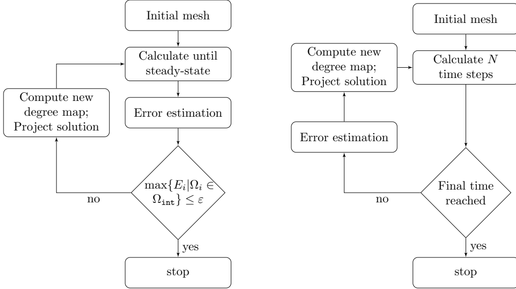
Figure 2: Adaptive strategy for steady-state solutions (left) and for transient solutions (right).
