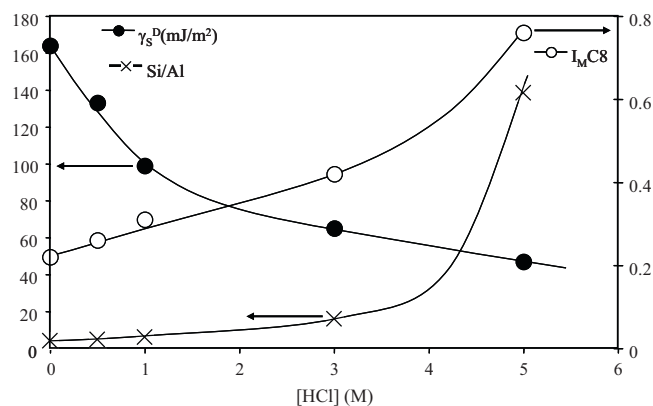
Fig. 8. Evolution of the dispersive component \gamma_s^d , the nanomorphological index I_M(\chi_t) , and the Si/Al ratio of attapulgite treated with HCl acid at different concentrations.
