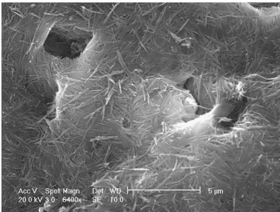
Fig. 3. SEM micrography of a hole appearing in attapulgite structure after acid treatment with 0.5 M HCl.
