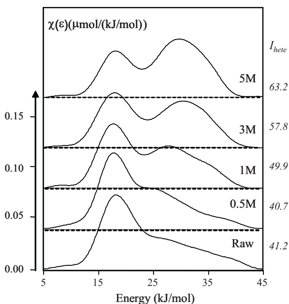
Fig. 11. Adsorption energy distribution functions of the isopropanol probe of the initial and treated attapulgite, measured at 43 °C.
