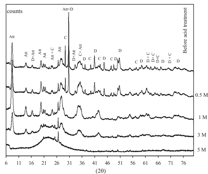
Fig. 5. XRD diffractograms of attapulgite before and after acid activation at different HCl concentrations (Att = attapulgite, D = dolomite, C = calcite).
