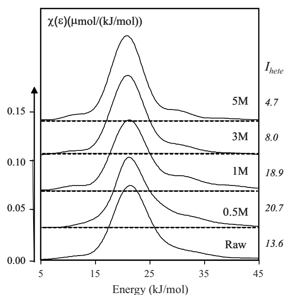
Fig. 10. Adsorption energy distribution functions of the n-octane probe of the initial and treated attapulgite, measured at 53 °C.
