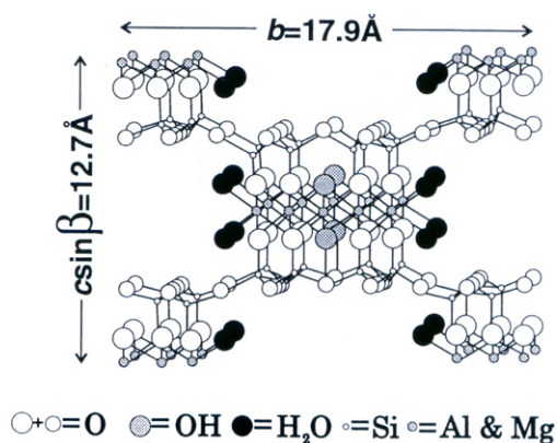
Fig. 1. Crystal structure of attapulgite [21].
