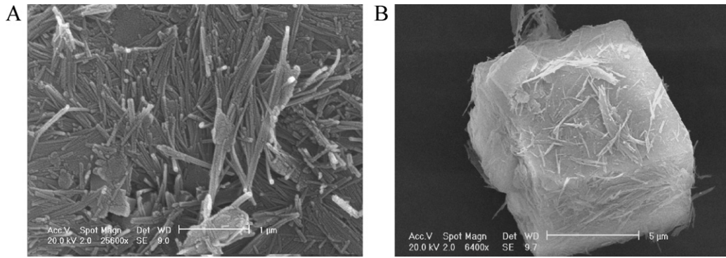
Fig. 2. SEM microographies of (A) attapulgite fibers and (B) a carbonate inclusion.
