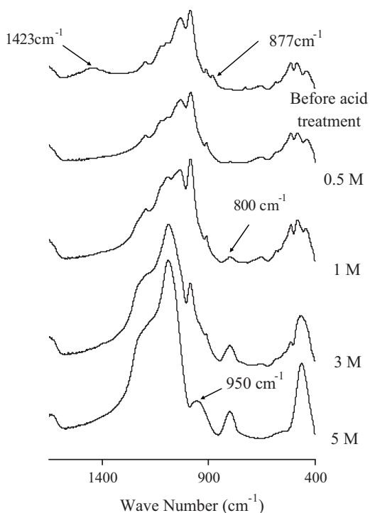
Fig. 7. FTIR spectra of attapulgite before and after treatment with HCl, in the 1500–400 \text{cm}^{-1} region.
