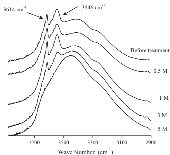
Fig. 6. FTIR spectra of attapulgite before and after treatment with HCl, in the 3800–2900 \text{cm}^{-1} region.
