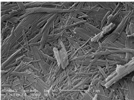
Fig. 4. SEM micrography of attapulgite, after treatment with 5 M HCl.
