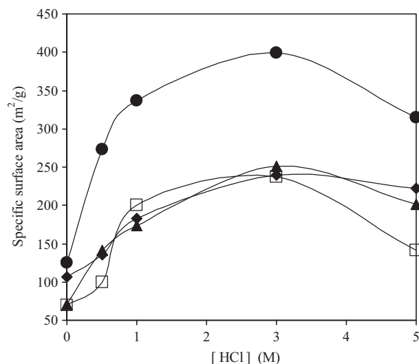
Fig. 9. Evolution of the specific surface area of attapulgite treated with various concentrations of HCl, measured by nitrogen adsorption ● and IGC-FC with octane ◆, isopropanol □, and dioxan ▲.
