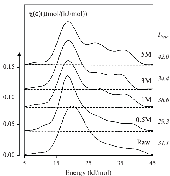
Fig. 12. Adsorption energy distribution functions of the dioxan probe of the initial and treated attapulgite, measured at 51 °C.
