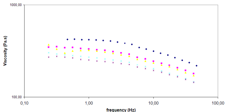
FIGURE 1. Melt rheology of PEEK
