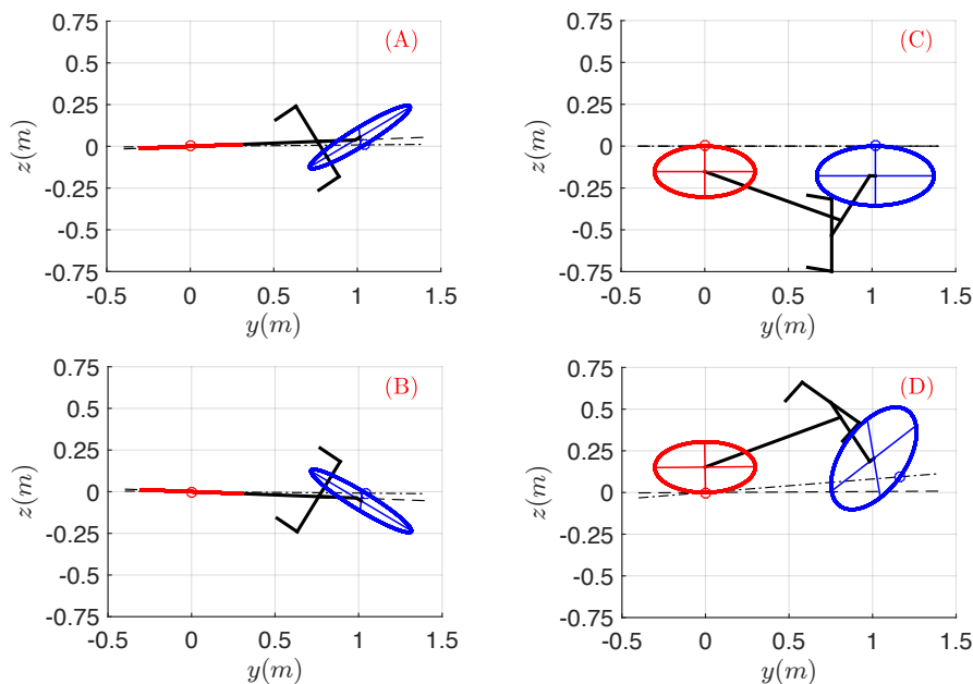
Figure 9: Top views to the bicycle when (\phi_0, r_1) = (0, 30) (A), (0, -30) (B), (30, 0) (C) and (-30, 45) , all angles being in degrees. (---) line of contact points on the ground. (- · -) projected line of the rear-wheel plane onto the ground.
