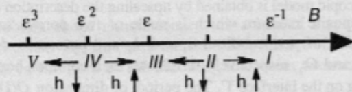
Figure 1. The different macroscopic models
