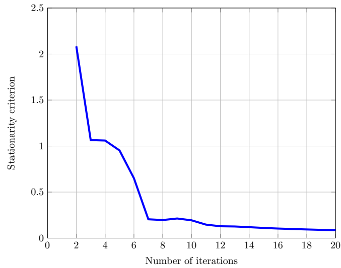
Fig. 5 – Evolution of sub-iteration number necessary to reach a stationarity criteria
