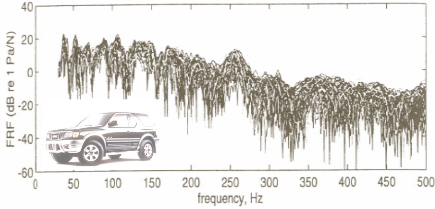
Fig. 1 – Frequency response of 98 “identical” cars from the same production line (courtesy of Toyota) [1]
