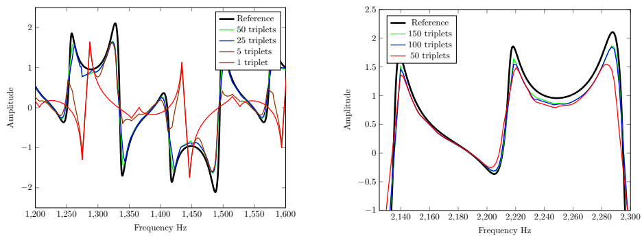
(a) Solution reconstruction for different PGD approximation orders (b) Zoom on the peaks to show high order contributions
