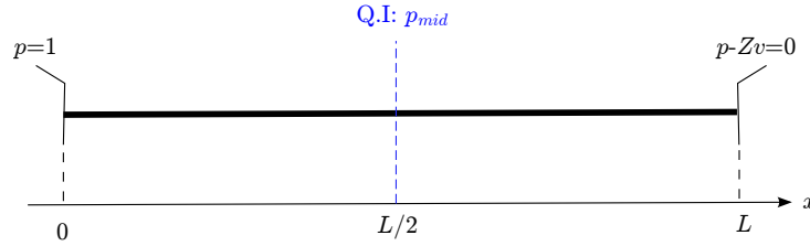
Fig. 2 – 1D problem
