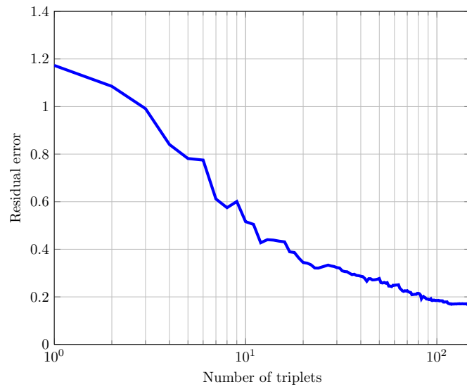
Fig. 4 – Residual error
