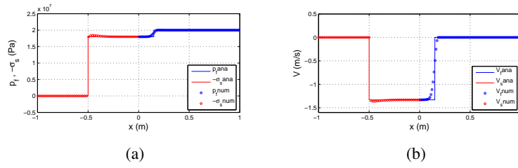
Fig. 8: Comparison with the analytical solution (Explicit Newmark scheme).
