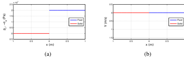
Fig. 6: Initial configuration for the test case with 1D linear beam: (a) initial profile of fluid pressure ( p_f ) and solid stress ( -\sigma_s ); (b) initial profile of fluid and solid velocity.
