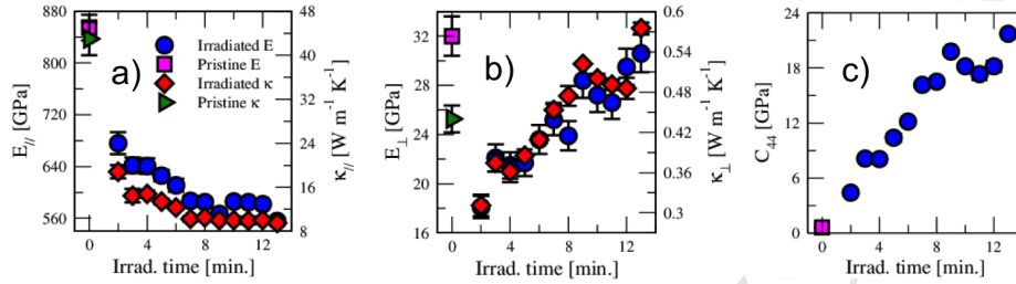
Figure 10: Evolution with irradiation time of (a) the longitudinal and (b) transverse Young's moduli and thermal conductivities as well as of (c) the basal shear elastic constant ( C_{44} ). Values and error bars of E_{\parallel} and \kappa_{\parallel} for the IGAR models are based on the average values and deviations, respectively, from simulations performed along x and y directions.
