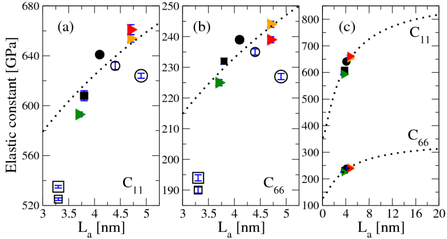
Figure 3: Same as Fig. 2 for the evolutions of C_{11}^T (a) and C_{66}^S (b) with L_a .
