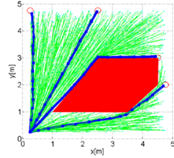
Fig. 5. Multi-RRT*FN based path planning.
