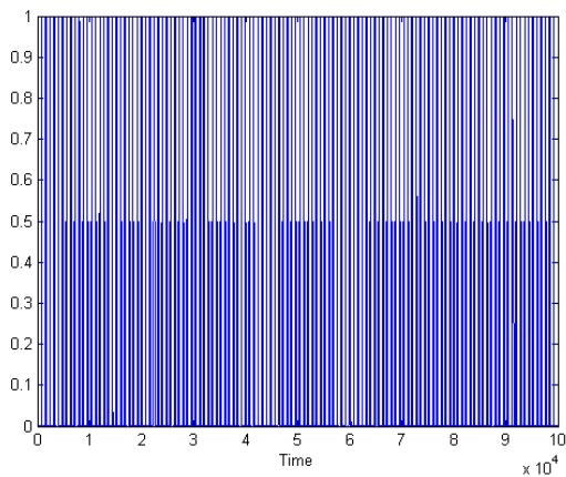
FIGURE 3 – estimated \zeta(k)
