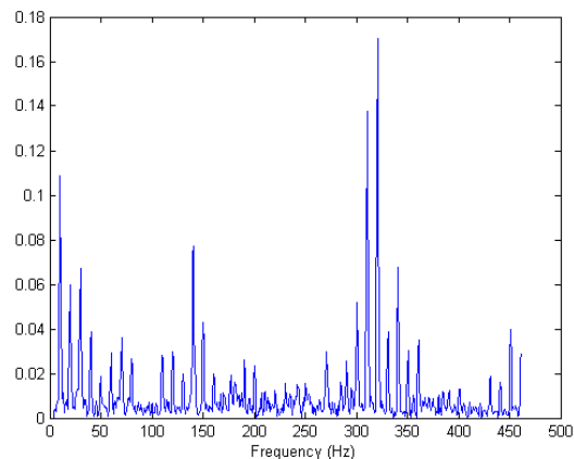
FIGURE 6 – Envelope spectrum
