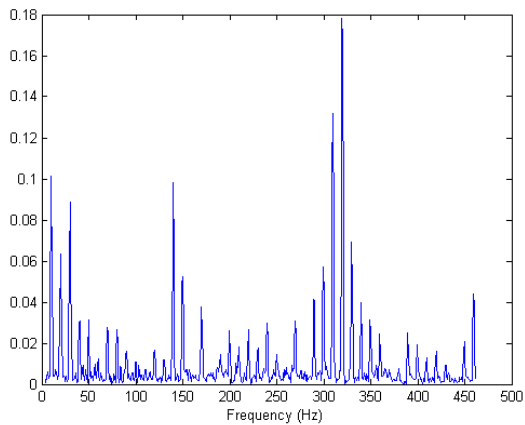
FIGURE 10 – Envelope spectrum
