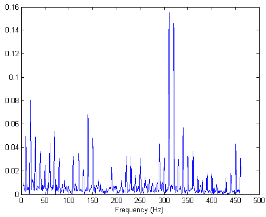
FIGURE 8 – Envelope spectrum
