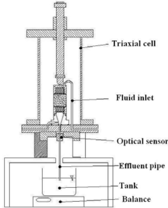
Figure 1: Schematic diagram of the triaxial erodimeter.
