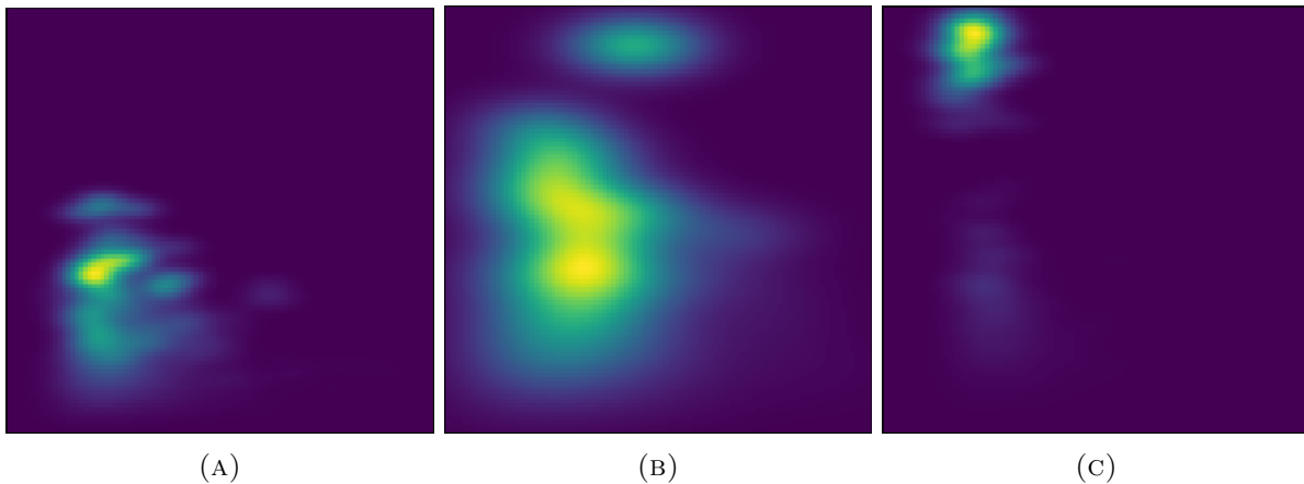
FIGURE 4. Persistence surfaces for each class (a), (b) and (c), computed with the weight function w(\mathbf{r}) = (r_2 - r_1)^3 and with the bandwidth matrix selected by the cross-validation procedure.
