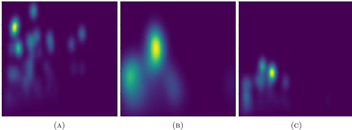
FIGURE 5. Persistence surfaces for each person A,B and C, computed with the weight function w(\mathbf{r}) = (r_2 - r_1)^3 and with the bandwidth matrix selected by the cross-validation procedure.
