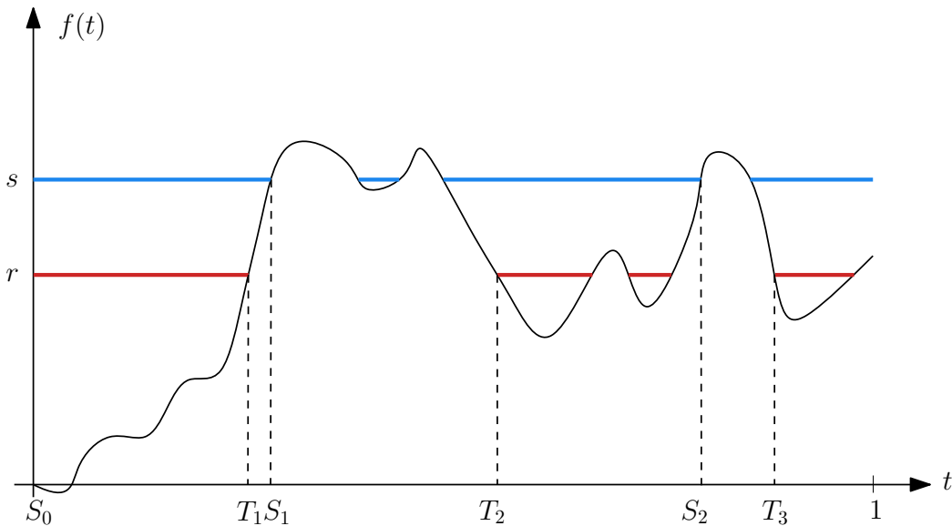
FIGURE 1. Example of a function f : [0, 1] \rightarrow \mathbb{R} with \beta^{r,s} = 3 . The red region corresponds to f^{-1}((-\infty, r]) and the blue region to f^{-1}((-\infty, s]) .
