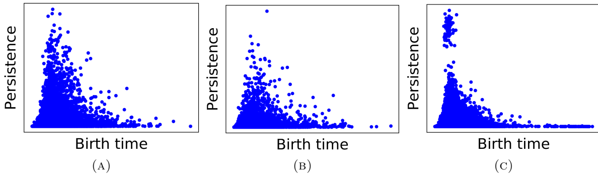
FIGURE 3. Superposition of the N = 40 diagrams of class (a), (b) and (c), transformed under the map \mathbf{r} \rightarrow (r_1, r_2 - r_1) .
