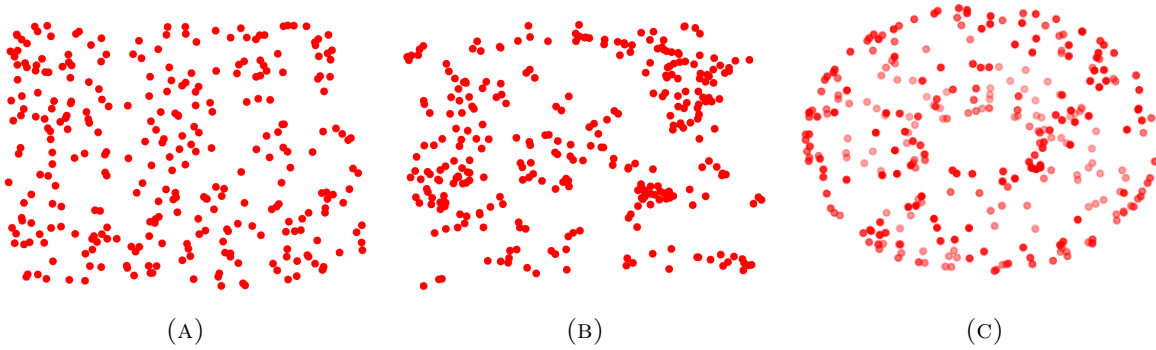
FIGURE 2. Realization of the processes (a), (b) and (c) described in Section 9.
