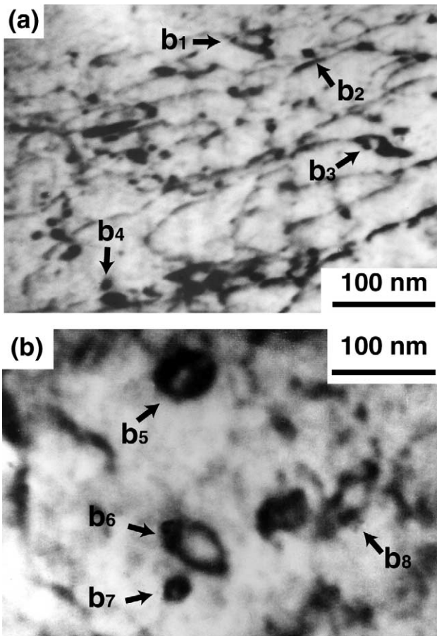
Fig. 5. TEM bright field images extracted from in situ straining sequences at (a) -123\text{ }^{\circ}\text{C} and (b) +130\text{ }^{\circ}\text{C} .
