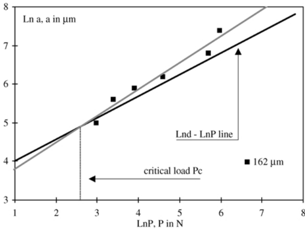
Figure 4 Principle for the determination of the critical load to initiate interface cracking by Vickers indentation illustrated for 162 \mu\text{m} thick NiO (see text for detail).
