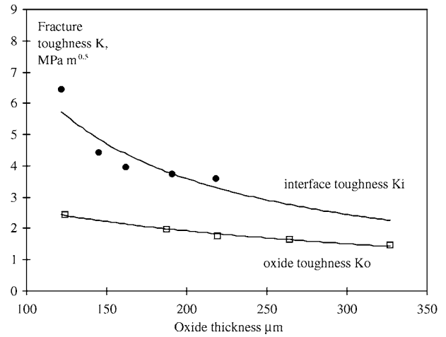
Figure 6 Comparative evolution of the interface and oxide fracture toughness versus oxide thickness.
