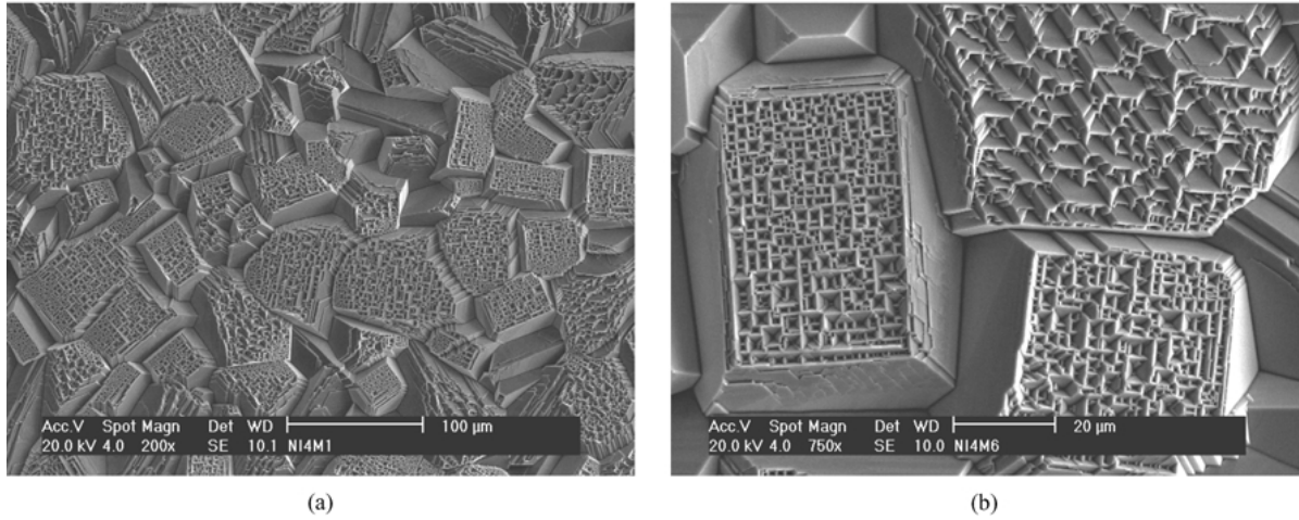
Figure 1 Morphology of the nickel oxide after isothermal oxidation at 1200 °C for 408 h, low magnification SEM image (a) and detail of individual oxide grains (b).
