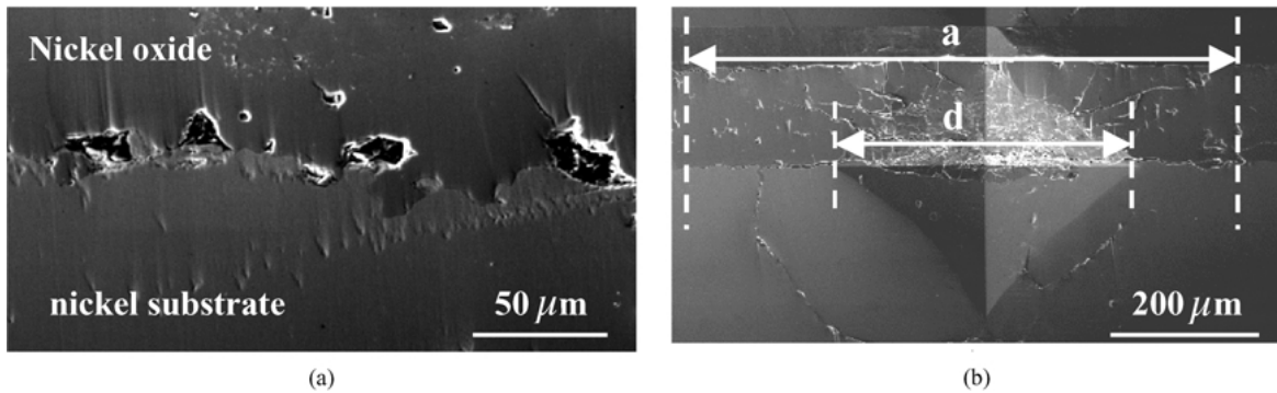
Figure 2 Morphology of the interface Ni/NiO after oxidation at 1200 °C for 288 h (a) and typical crack pattern after interface indentation of a specimen oxidized 192 h at 1200 °C ( a is the length of the indentation induced crack and d is the diagonal of the indentation imprint) (b).
