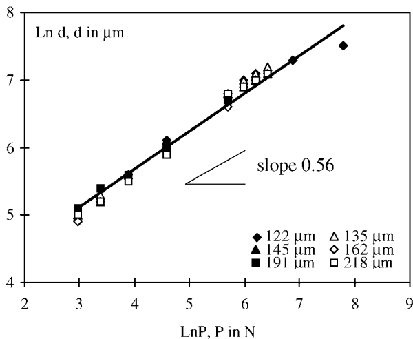
Figure 3 Diagonal of the indentation imprint d versus applied load P for various nickel oxide thicknesses ranging from 122 \mu\text{m} to 218 \mu\text{m} .
