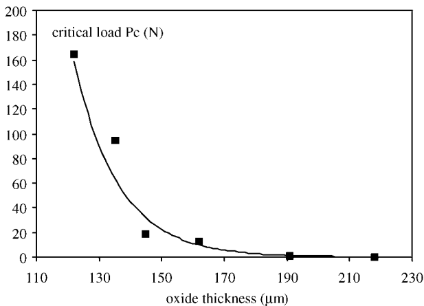
Figure 5 Variation of the critical load with oxide thickness.
