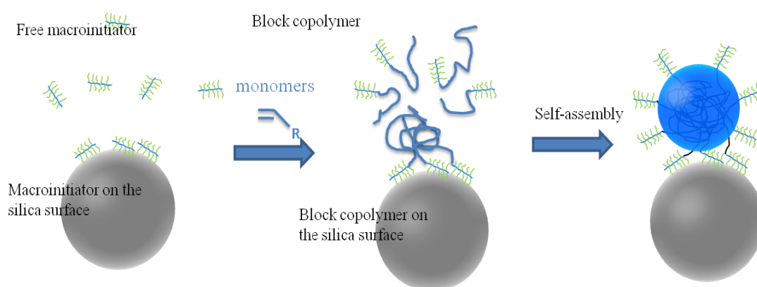
Scheme 2. Schematic illustration of the synthesis of multipod-like silica/polymer particles by NMP-mediated polymerization-induced self-assembly of block copolymers by means of a physically adsorbed brush-type macroalkoxyamine initiator.
