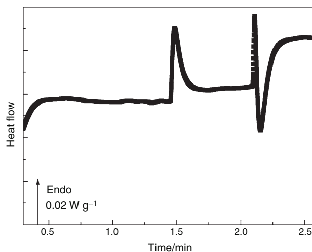
Fig. 2 Isotherm DSC response recorded for (VGGVG) 3 in pure water ( 10^{-3}\text{ g cm}^{-3} ) at 37\text{ }^{\circ}\text{C}
