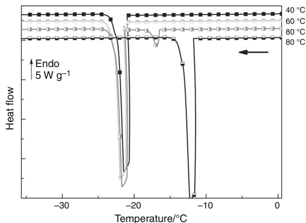
Fig. 4 DSC curves of (VGGVG) 3 in pure water ( 10^{-3} g cm −3 ) obtained with protocol B (temperatures noted in the right side indicate the final temperature of the heating ramp performed just before the cooling ramp). The length of the vertical arrow corresponds to the scale
