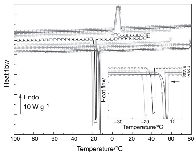
Fig. 3 DSC curves of (VGGVG) 3 in pure water ( 10^{-3} g cm −3 ) obtained with protocol A (temperatures noted in the right side indicated the final temperature of the heating ramp performed just before the cooling ramp). The length of the vertical arrow corresponds to the scale
