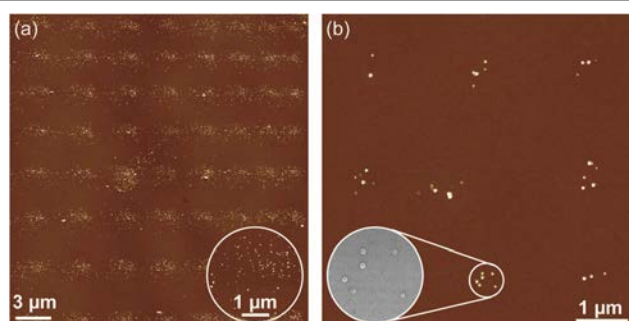
Fig. 2 (a) AFM image of an array of 64 spots obtained with a NADIS tip with a diameter of 760 nm; inset: zoom on one spot. (b) Same with a NADIS tip of 300 nm diameter.
