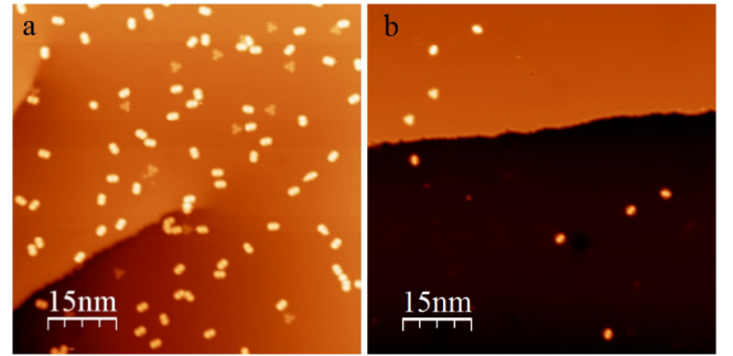
FIG. 2. STM image 75 \times 75 nm 2 of the \text{Ru}(\text{dbm})_3 molecules after evaporation on (a) the Ag(111) and (b) Cu(111) substrate held at low temperature ( V_s = -1 V, I_t = 1 pA, T = 4.5 K).
