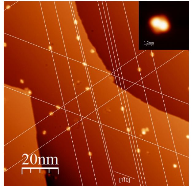
FIG. 3. Orientation of the bi-lobe structure on Cu(111). The orientation of the top ligand of most of the molecules are represented with white lines. Insert : Close up view ( 5 \times 5 nm 2 ) of the bi-lobe structure called B . ( V_s = 1.5 V, I_t = 15 pA, T = 4.5 K)
