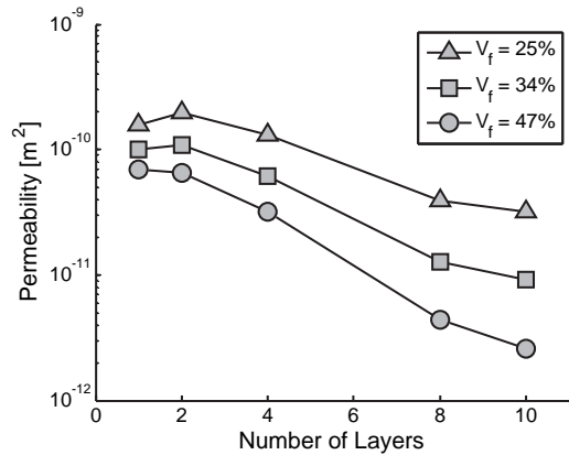
Figure 19. PW multi-layer through-thickness permeability test results.
