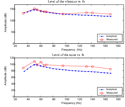
Figure 2: Comparative results of the noise and vibration of the asynchrone machine.
