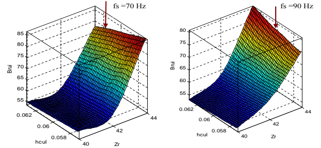
Figure 6: Surface response in noise function rotor slots number and height of yoke.
