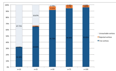
Fig. 4. Percentage of unreachable, rejected, and tree vertices.
