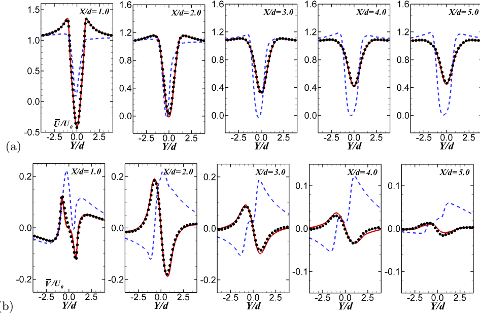
Figure 9: Mean velocity profiles along the height of the plate (● Narasimhamurthy & Andersson (2009), — LES normal ( 90^\circ ) and - - LES oblique ( 45^\circ )) at various X/d downstream locations: (a) Stream-wise velocity ( \bar{U}/U_0 ). (b) Cross-stream velocity ( \bar{V}/U_0 ).
