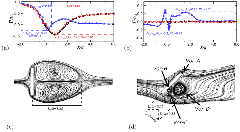
Figure 7: ● Narasimhamurthy & Andersson (2009), □ LES Normal ( 90^\circ ) case, \Delta LES oblique ( 45^\circ ) case: (a) Mean profile for stream-wise velocity ( \bar{U}/U_0 ). (b) Mean profile for cross-stream velocity ( \bar{V}/U_0 ). (c) Mean streamlines, LES Normal ( 90^\circ ) case. (d) Mean streamlines, LES oblique ( 45^\circ ) case.
