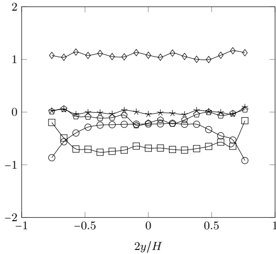
Figure 16: Budget analysis of the transport equation of q_p^2 given by Eq. (8). The symbols are \diamond : -1/(2n_p) \partial(n_p S_{p,ykk})/\partial y ; \square : -R_{xy} \partial U_{p,x} / \partial y ; \circ : \langle a_k^f u'_{p,k} \rangle_p ; \triangle : C(u'_{p,k} u'_{p,k}) / (2n_p) ; \star : sum of all terms.
