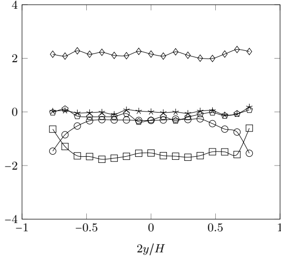
Figure 12: Budget analysis of the transport equation of R_{p,xx} given by Eq.(4). The symbols are \circ : -1/n_p \partial (n_p S_{p,yyx}) / \partial y ; \diamond : -2R_{xy} \partial U_{p,x} / \partial y ; \square : 2(a_x^f u'_{p,x})_p ; \star : sum of all the terms.
