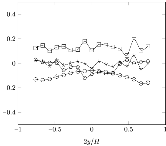
Figure 13: Budget analysis of the transport equation of R_{p,yy} given by Eq.(5). The symbols are \circ : -1/n_p \partial (n_p S_{p,yyy}) / \partial y ; \diamond : -R_{p,yy} \partial U_{p,x} / \partial y ; \square : \langle a_x^f u'_{p,y} \rangle + \langle a_y^f u'_{p,x} \rangle_p ; \star : sum of all terms.
