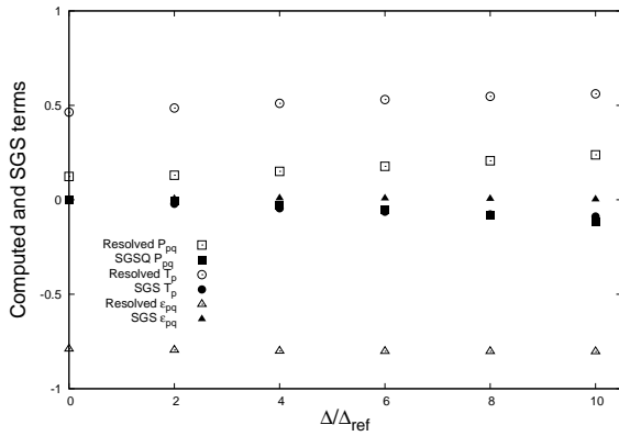
Figure 6: Resolved and sub-grid collision term contributions in the random particle kinetic energy filtered transport equation for d_p = 75 \mu m for various filter widths \Delta (normalized by \tilde{\alpha}_p \rho_p V_{p,St}^2 / \tau_{p,St} )
