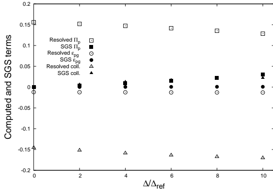
Figure 5: Resolved and sub-grid contributions in the random particle kinetic energy filtered transport equation for d_p = 150 \mu m for various filter widths \Delta (normalized by \tilde{\alpha}_q \rho_q V_{q,St}^2 / \tau_{q,St} )
