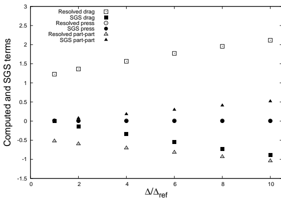
Figure 2: Resolved and sub-grid contributions in the particle momentum filtered transport equation for d_p = 75 \mu m for various filter widths \Delta (normalized by \tilde{\alpha}_p \rho_p g_z )
