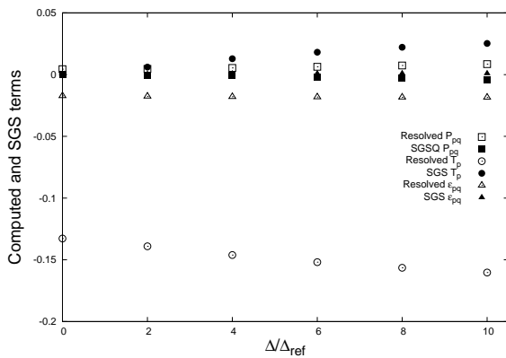
Figure 7: Resolved and sub-grid collision term contributions in the random particle kinetic energy filtered transport equation for d_p = 150 \mu m for various filter widths \Delta (normalized by \tilde{\alpha}_q \rho_q V_{q,St}^2 / \tau_{q,St} )
