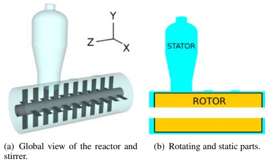
Figure 8: View of the geometry.
