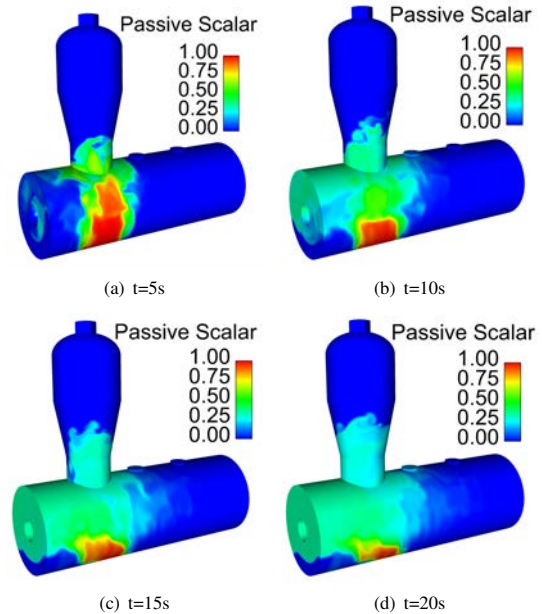
Figure 13: Transport of a passive scalar by the gas phase at four consecutive times.
