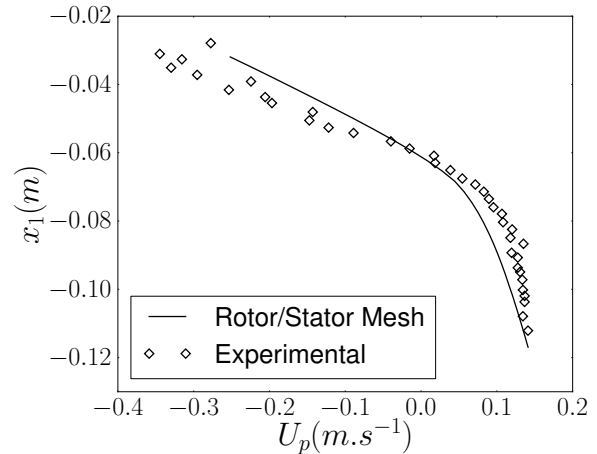
Figure 5: Comparison of velocity profiles in the depth of the particle bed.
