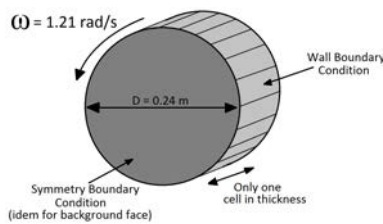
(a) Sketch of the drum
