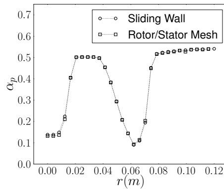
Figure 2: Comparison of solid volume fractions at t = 30\text{s} .
