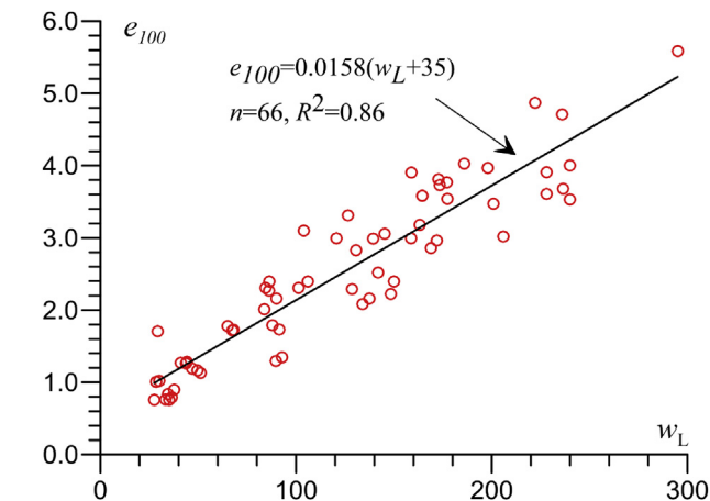
Fig. 13. Relationship between the void ratio at 100 kPa and the liquid limit.
