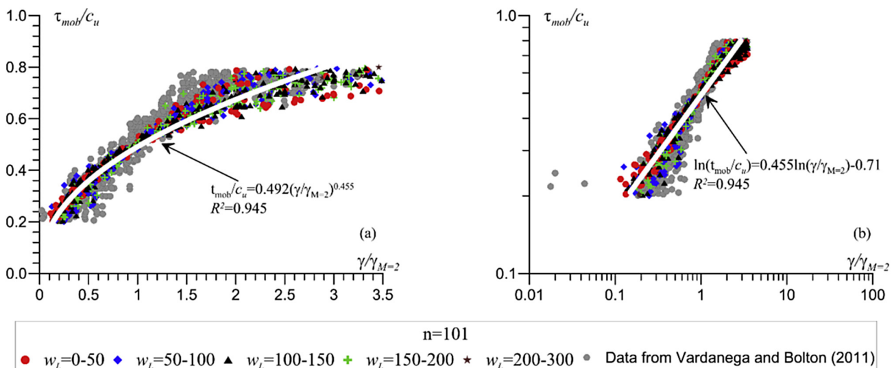
Fig. 19. Normalized shear stress and shear strain based on the results of undrained triaxial tests.
