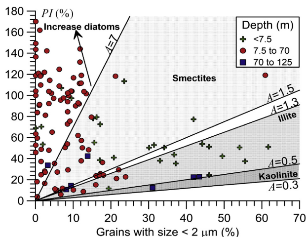
Fig. 6. Activity plot of clay content (grains with sizes smaller than 2 \mu m) and plasticity index for the Bogotá clays.
