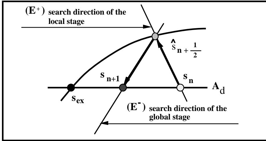
Figure 1: Iteration scheme
