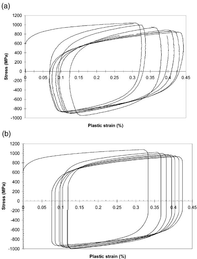
Fig. 13. Non symmetrical total strain ( -0.5/+1\% ) fatigue test at 500^\circ\text{C} . Stress–plastic strain loops 1, 5, 10, 50, 100, 500, 1000. (a) Experimental, (b) model response.
