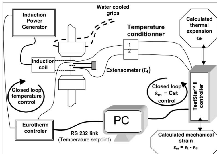
Fig. 6. TMF experimental test equipment.
