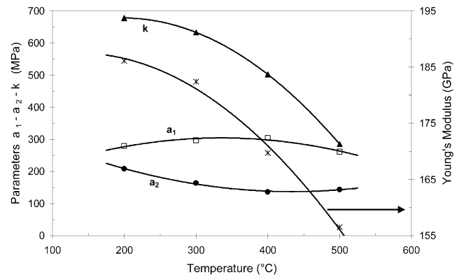
Fig. 12. Quadratic evolution of model parameters a_1 , a_2 , k and E .
