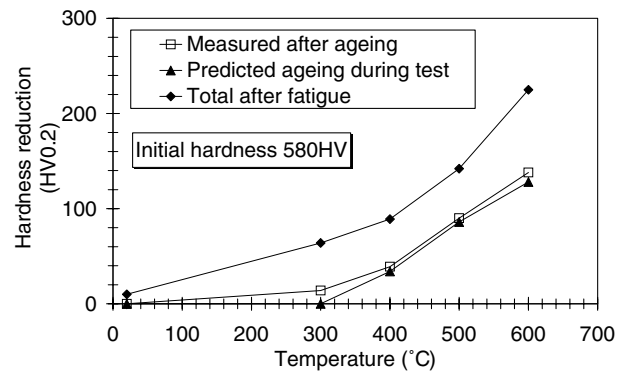
Fig. 12. Comparison between the hardness decrease measured after fatigue and ageing tests (same conditions of time and temperature) and the corresponding calculated value from Eq. (4).
