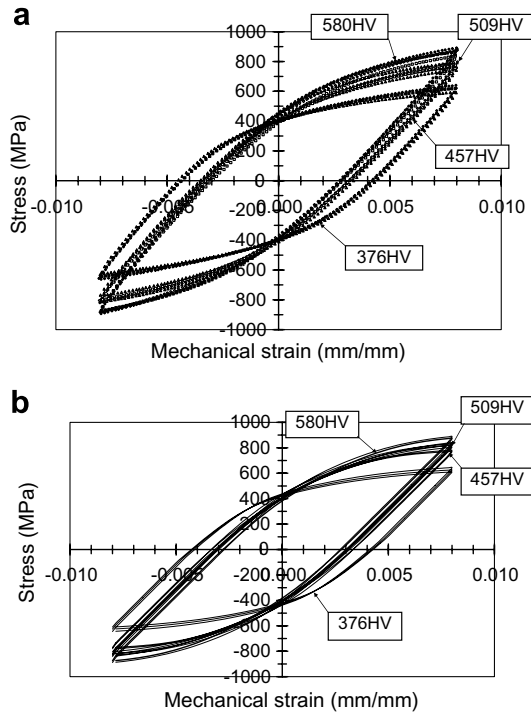
Fig. 6. Stress-strain loops at 500 °C for three strain rates ( 10^{-2} s^{-1} , 10^{-3} s^{-1} , 10^{-4} s^{-1} ) and for the four investigated initial hardness ( \Delta\epsilon_t = \pm 0.8\% ): (a) experimental, (b) simulation.
