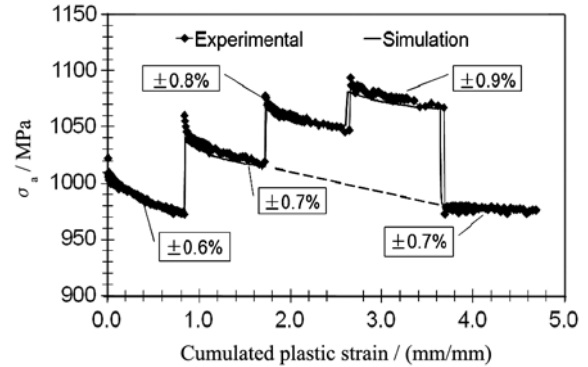
Fig. 4. Experiment-simulation comparison: stress amplitude-cumulated plastic strain for a type two test on sample 45.5HRC tested at 573 K.
