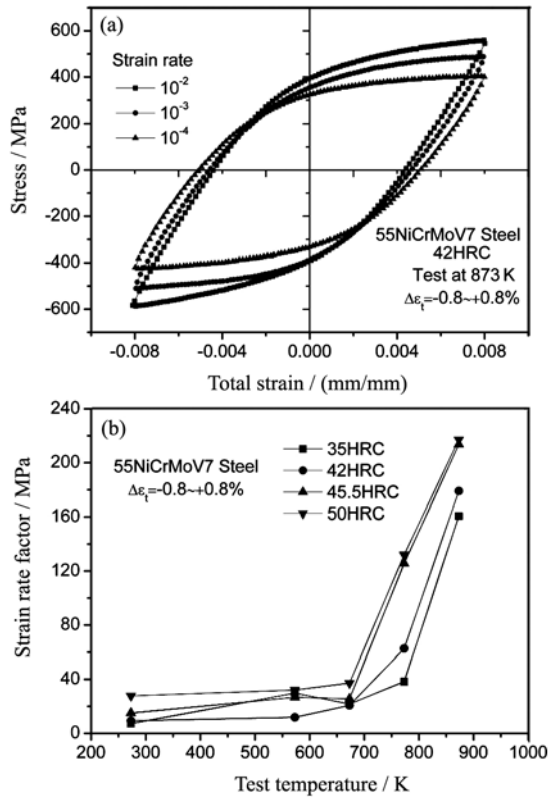
Fig. 2. (a) Stress-strain hysteresis loops at different strain rates, (b) F-T curves of the steel 55NiCrMoV7.
