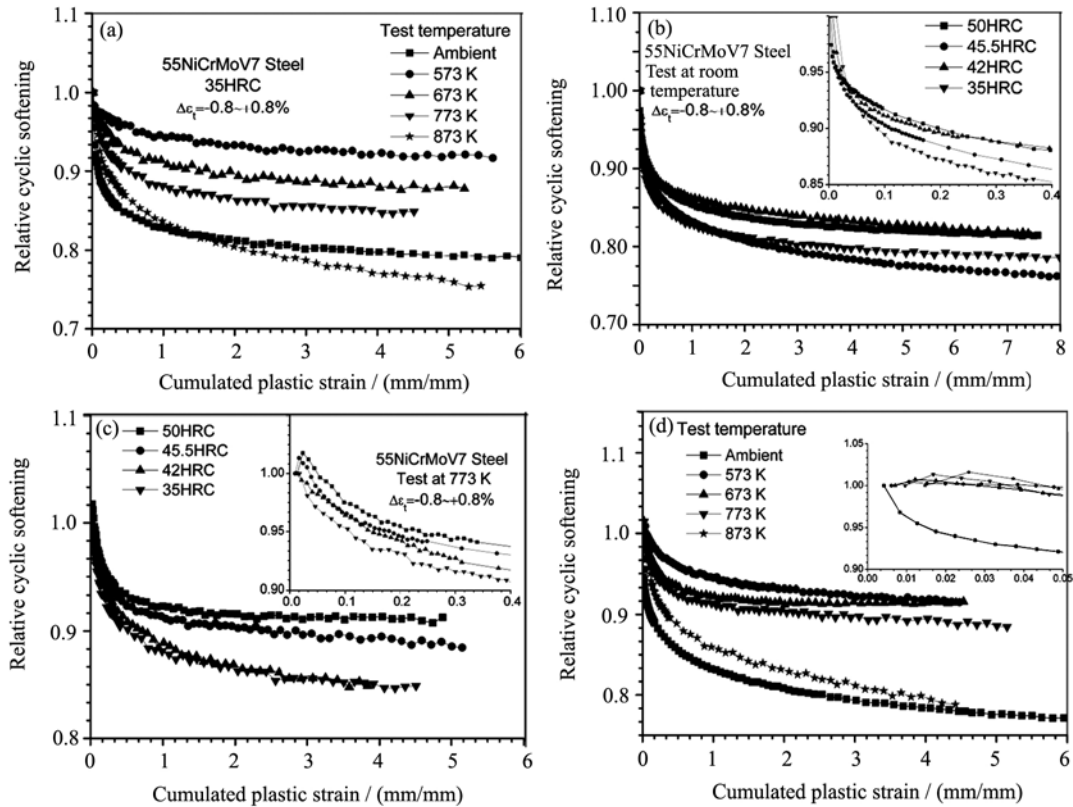
Fig. 1. \Delta\sigma_i/\Delta\sigma_1 - p curves of steel: (a) 35HRC, (b) at ambient, (c) at 773 K, (d) 45.5HRC.
