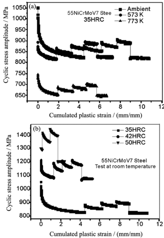
Fig. 3. Multi-levels \sigma - p curves of steel 55NiCrMoV7: (a) 35HRC, (b) at room temperature.
