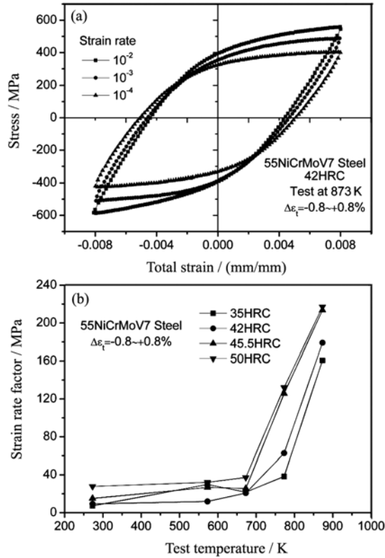
Fig. 2. (a) Stress-strain hysteresis loops at different strain rates, (b) F-T curves of the steel 55NiCrMoV7.
