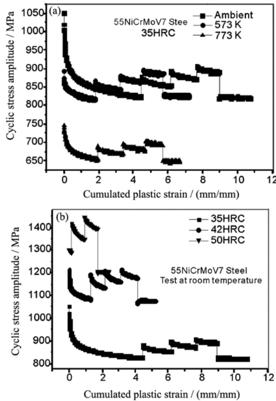
Fig. 3. Multi-levels \sigma - p curves of steel 55NiCrMoV7: (a) 35HRC, (b) at room temperature.
