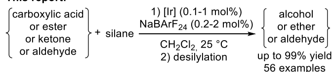
Scheme 1. Hydrosilylation of carboxylic acid derivatives using an iridium(III) metallacycle.
