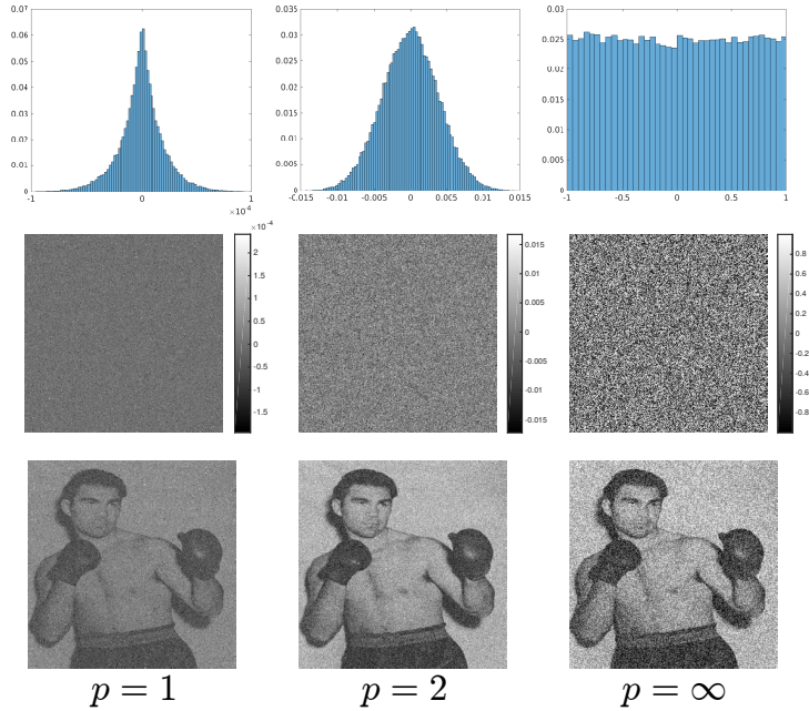
Figure 1: Illustration of noise with different values of p . First row: histogram of uniformly sampled noise from the unit ball of \ell_p^d . Second row: Example of noise image. Third row: Example of noisy image. Note that different values of p result in perceptually different noise images.
