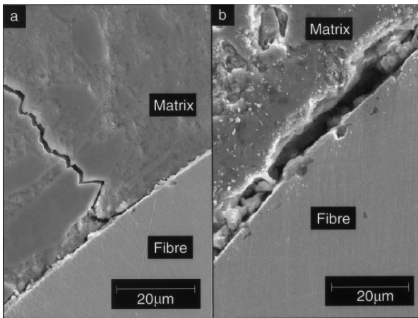
Fig. 4. SEM micrographs of fibre/matrix interfaces after a 500 °C firing treatment.
