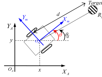
Fig. 2 Robot configuration in a Cartesian reference frame.
