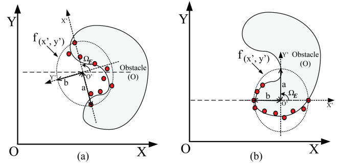
Fig. 6. Obtained ellipse using heuristic approach for two data set of points.
