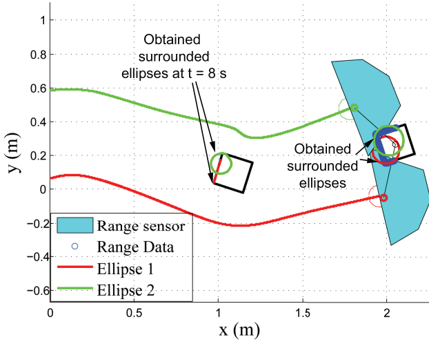
Fig. 9. Navigation of the multi-robot formation using object detection of each robot separately.
