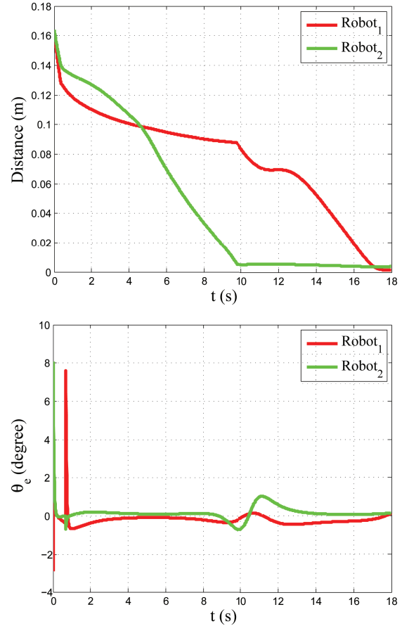
Fig. 12. Distance and orientation error of the multi-robot formation.
