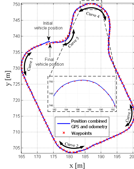
Fig. 10. GPS real Trajectory of the vehicle and waypoints.
