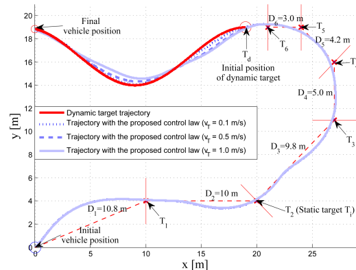
Fig. 5. Trajectories of the vehicle for several target velocities.
