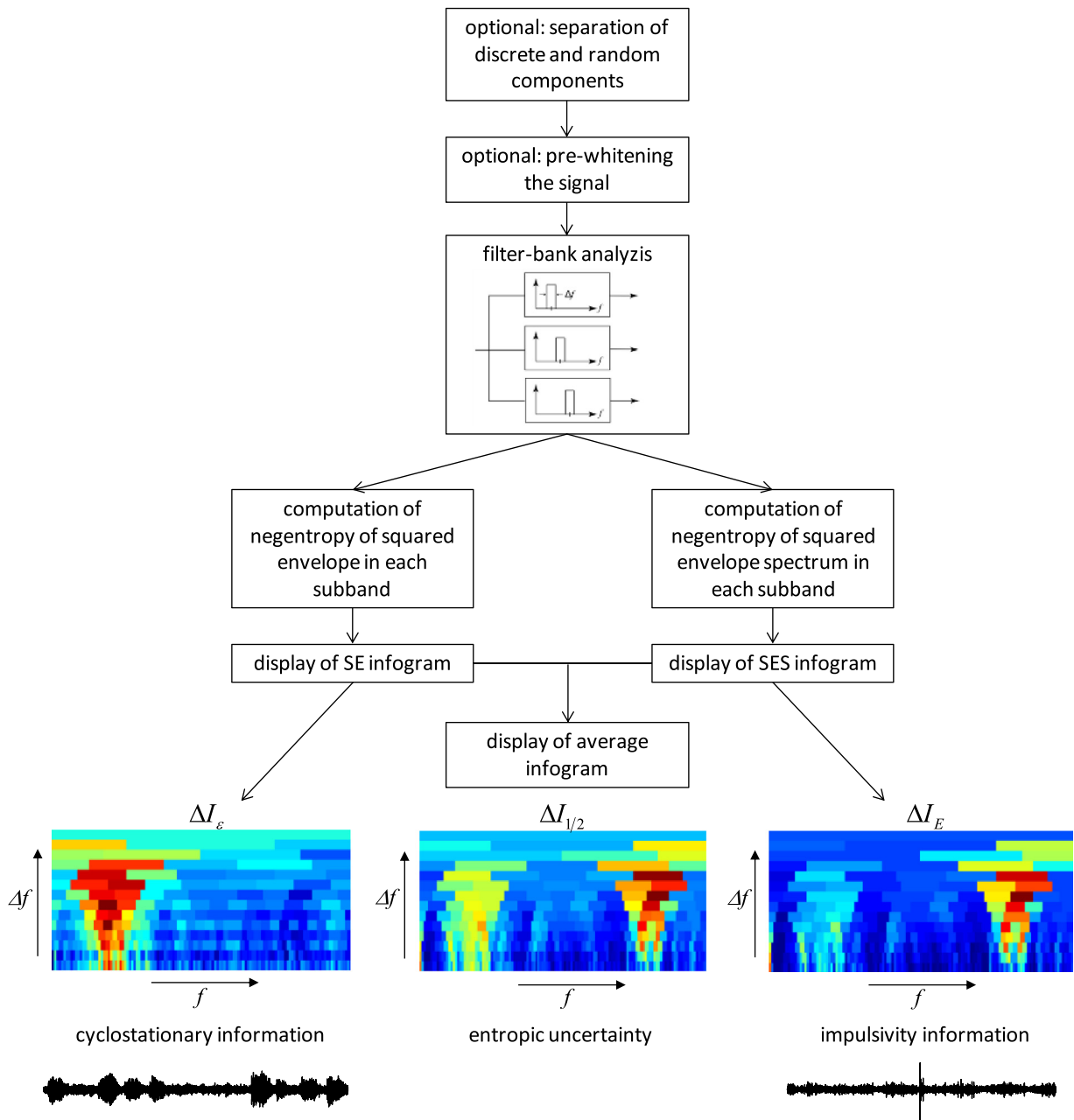
Fig. 5. Flowchart of the algorithm for computing the infograms.
