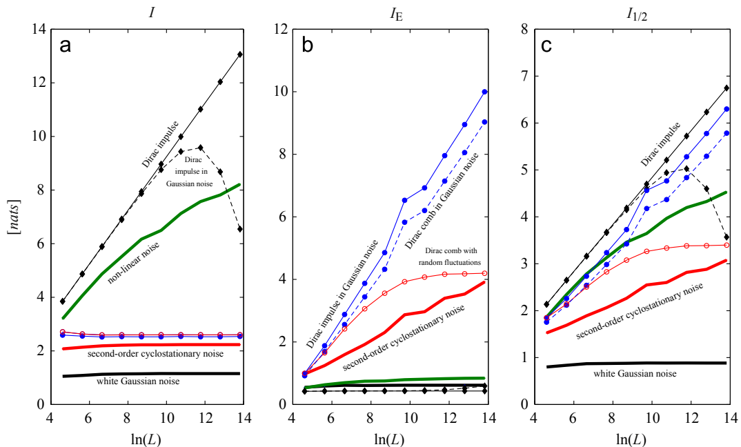
Fig. 4. Spectral negentropies: (a) \Delta I_\varepsilon , (b) \Delta I_E and (c) their average \Delta I_{1/2} = (\Delta I_\varepsilon + \Delta I_E)/2 in full band \Delta f = F_s . Black thick line: white Gaussian noise; green thick line: non-linear noise; Red thick line: second-order cyclostationary noise ( N = 30 ); black line with diamonds: Dirac impulse; black dotted line with diamonds: Dirac impulse in Gaussian noise (crest-factor=50); blue line with circles: Dirac comb ( N = 30 ); blue dotted line with circles: Dirac comb in Gaussian noise ( N = 30 , SNR=20 dB); red line with circles: Dirac comb with 3% random fluctuations around the mean period N = 30 . (For interpretation of the references to color in this figure legend, the reader is referred to the web version of this article.)
