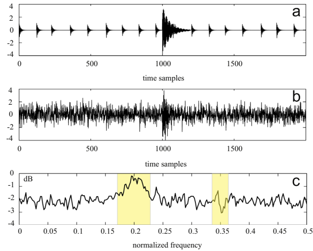
Fig. 6. (a) Synthetic signal simulating the series of transients produced by a faulty rolling element bearing and further corrupted by impulsive noise at time instant n = 1000 . (b) Same signal in additive white Gaussian noise (SNR = -12 dB). (c) Power spectral density of noisy signal (frequency resolution = 0.002) with highlights of the resonances at 0.2 and 0.35 that carry the series of transients and the impulsive noise, respectively.
