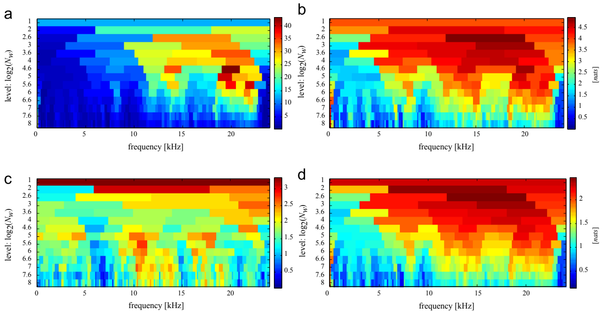
Fig. 14. Analysis of a vibration signal with an inner race fault. (a) Kurtogram, (b) SE infogram \Delta I_e(f; \Delta f) , (c) SES infogram \Delta I_E(f; \Delta f) , (d) average infogram \Delta I_{1/2}(f; \Delta f) .
