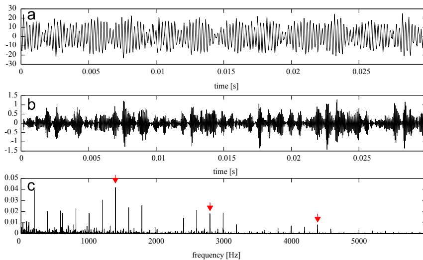
Fig. 19. (a) Faulty vibration signal and (b) its filtered version in band [18,000;23,000] Hz together with (c) its squared envelope spectrum. Inner race fault is diagnosed at 1400 Hz (note the strong modulation by shaft speed).
