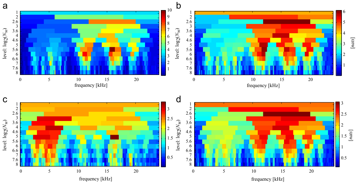
Fig. 16. Analysis of a vibration signal with an outer race fault: (a) Kurtogram, (b) SE infogram \Delta I_e(f; \Delta f) , (c) SES infogram \Delta I_E(f; \Delta f) , (d) average infogram \Delta I_{1/2}(f; \Delta f) .
