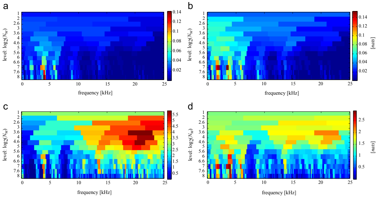
Fig. 18. Analysis of a vibration signal with a high-frequency inner race fault. (a) Kurtogram, (b) SE infogram \Delta I_e(f; \Delta f) , (c) SES infogram \Delta I_E(f; \Delta f) , (d) average infogram \Delta I_{1/2}(f; \Delta f) .
