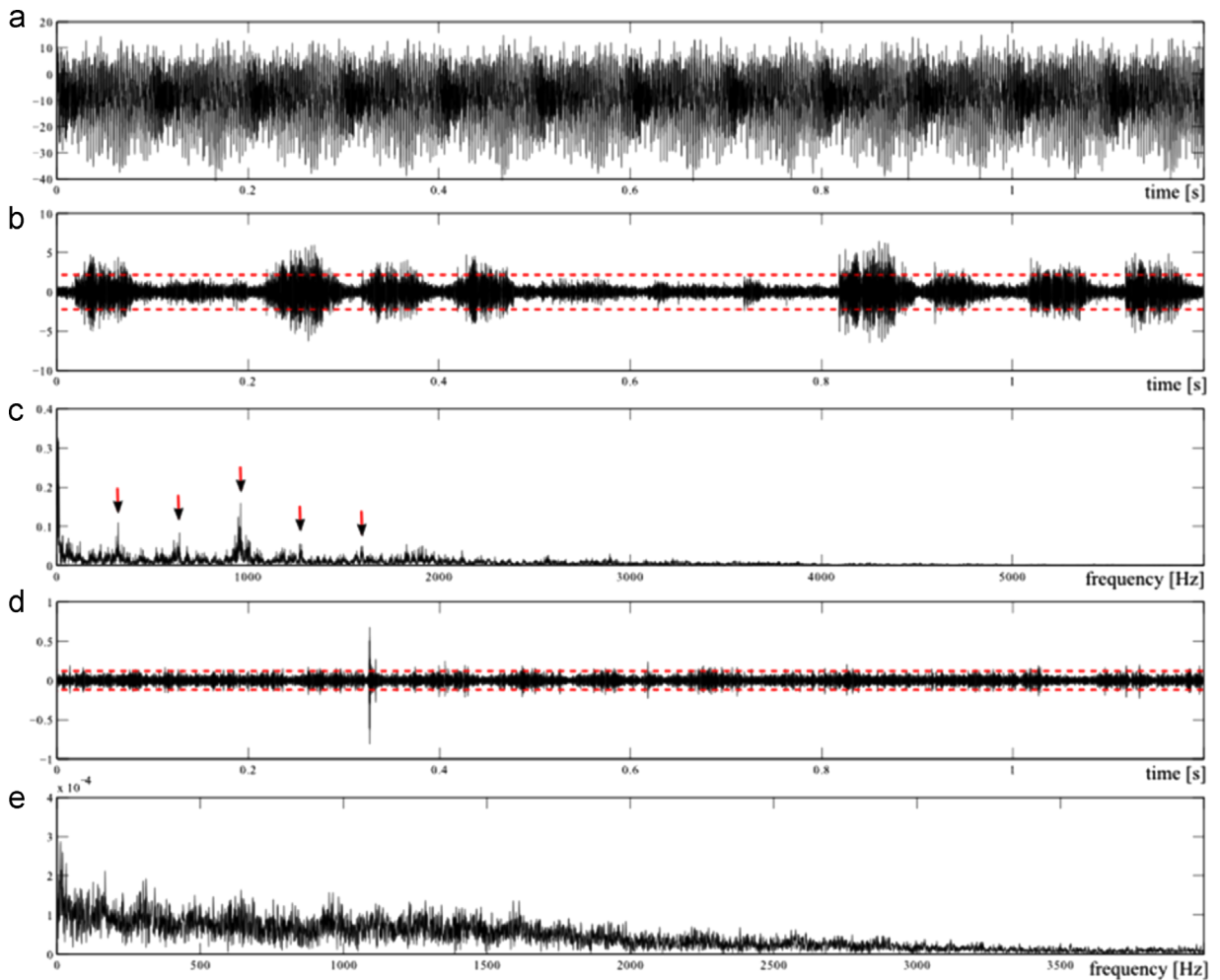
Fig. 13. (a) Healthy vibration signal and its filtered versions in bands (b) [4500;7500] Hz and (d) [19,750;20,250] Hz together with their respective squared envelope spectra (c) and (e).
