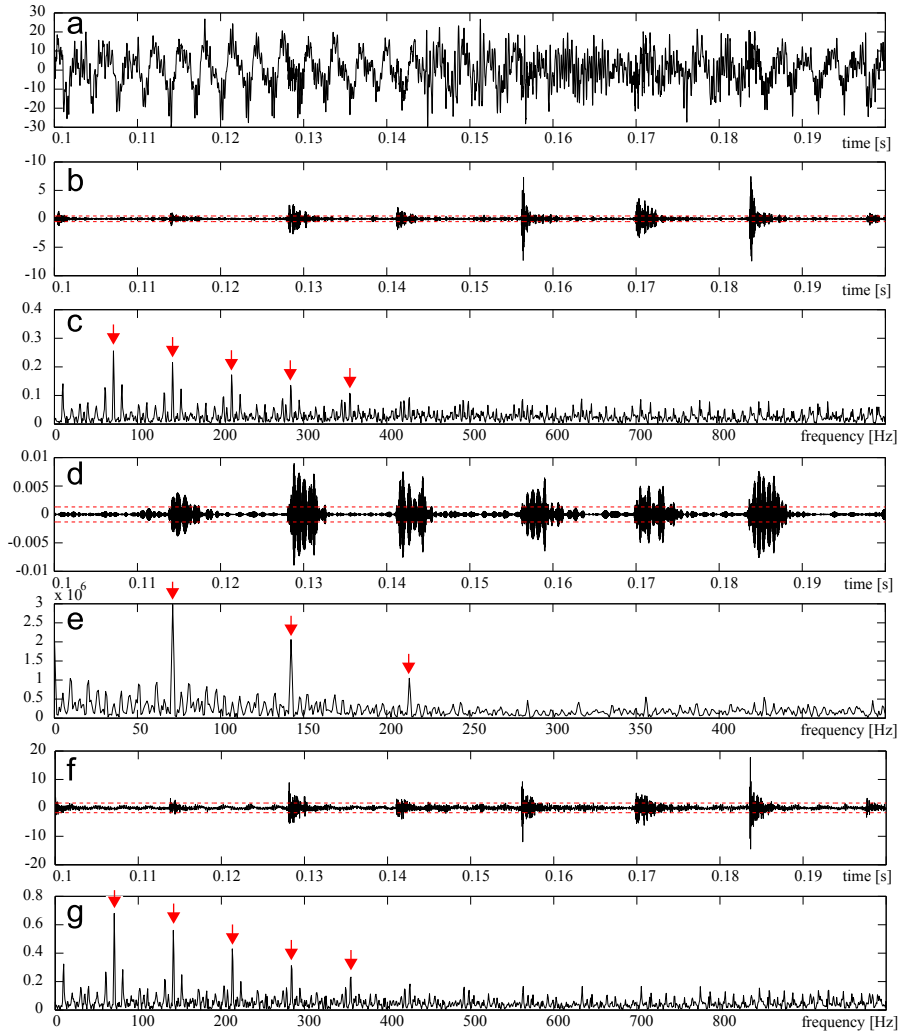
Fig. 15. (a) Faulty vibration signal (inner race fault) and its filtered versions in bands (b) [19,000;21,000] Hz, (d) [23,625;24,000] Hz, and (f) [9500;11,000] Hz together with their respective squared envelope spectra in (c), (e) and (g). Inner race fault is diagnosed at 71.12 Hz.
