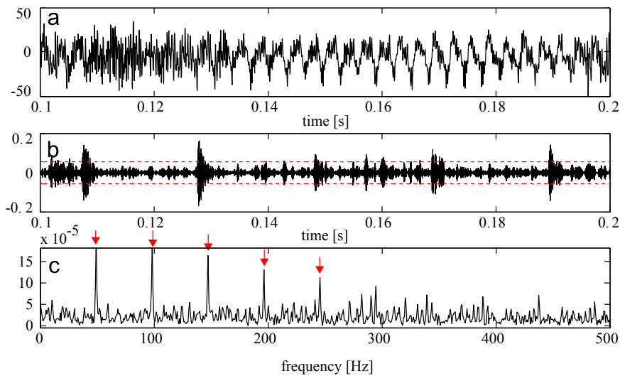
Fig. 17. (a) Faulty vibration signal (outer race fault) and (b) its filtered version in band [15,500;17,500] Hz together with (c) its squared envelope spectrum. Outer race fault is diagnosed at 49.10 Hz.
