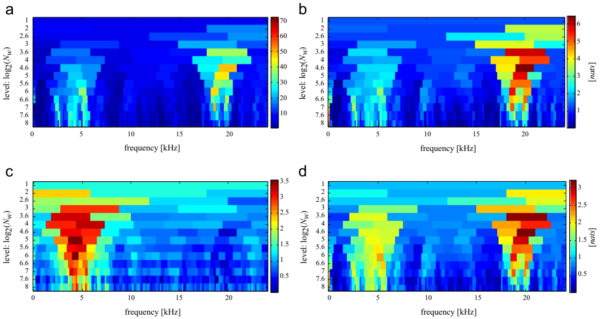
Fig. 12. Analysis of a vibration signal from a healthy bearing. (a) Kurtogram, (b) SE infogram \Delta I_e(f; \Delta f) , (c) SES infogram \Delta I_E(f; \Delta f) , (d) average infogram \Delta I_{1/2}(f; \Delta f) .
