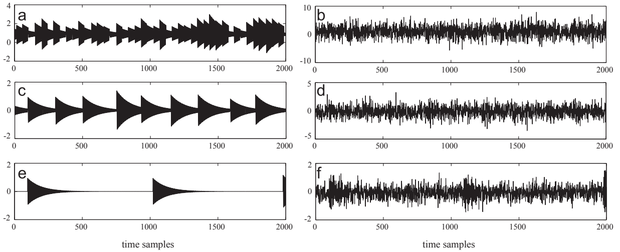
Fig. 8. Synthetic signals simulating the series of transients produced by a faulty rolling element bearing with mean period (a) N = 50 , (c) N = 200 , and (e) N = 1000 . (b, d and f) Corresponding signals after addition of white Gaussian noise with constant \text{SNR} = -6\text{dB} .
