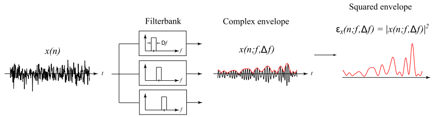
Fig. 2. Illustration of the concept of squared envelope as a mean of measuring the energy fluctuations in a signal (reproduced from Ref. [26]).
