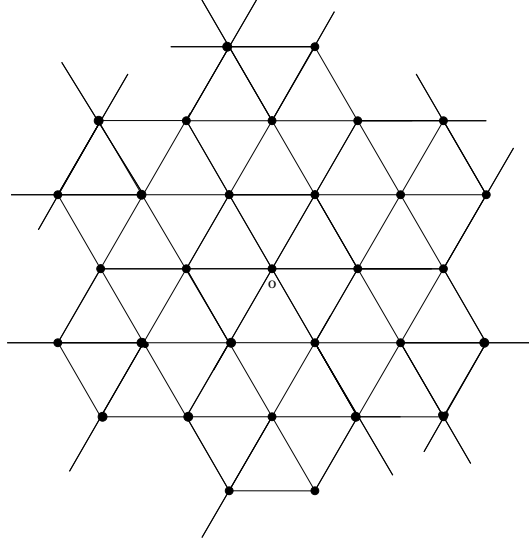
FIGURE 1. An infinite 6-regular triangulation
