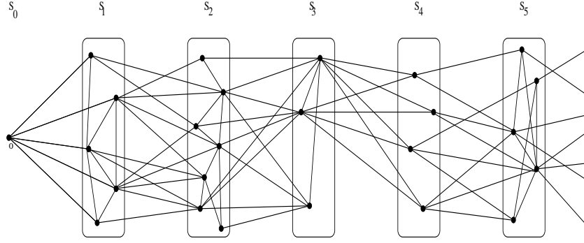
FIGURE 3. A triangulation with 1-dimensional decomposition
