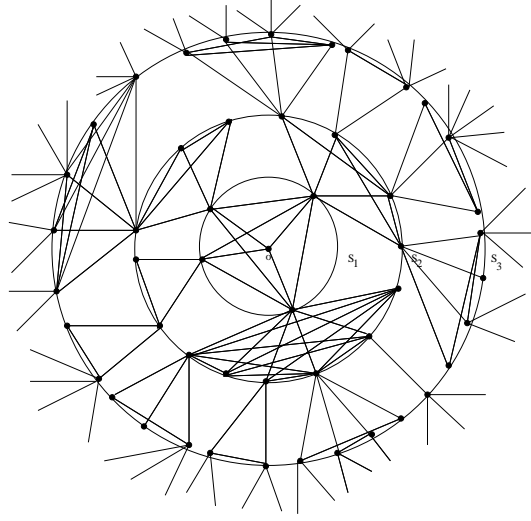
FIGURE 2. A Triangular Tree
