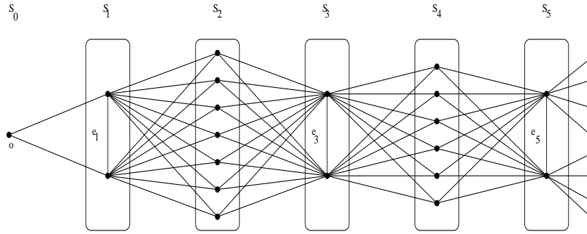
FIGURE 4. A particular triangulation with 1-dimensional decomposition
