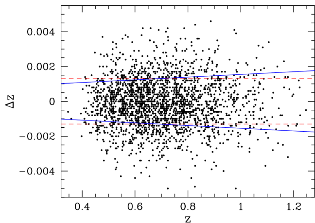
Fig. 10. Redshift measurement differences between two independent observations of the same object, obtained from a set of 2,466 VIPERS galaxies with quality flag \geq 2 , plotted as a function of the object redshift. Non-matching measurements (defined as being discrepant by more than |\Delta z| = 0.005 ) have been excluded from the plot. The dashed red and continuous blue lines show the 1-sigma scatter estimates obtained assuming the scatter to be independent from z , or scaling as (1+z) , respectively.
