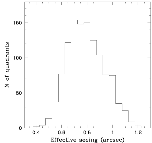
Fig. 1. The effective seeing distribution for the VIPERS observations. The seeing value is obtained from the measurement of the FWHM size of the spectral traces for bright objects in the spectroscopic exposures.
