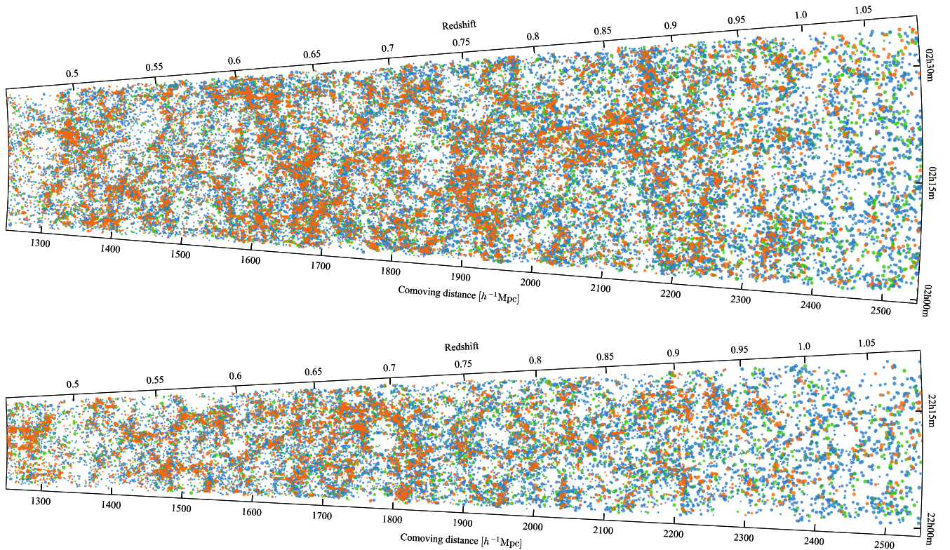
Fig. 14. The distribution of galaxies at 0.45 < z < 1.1 as shown by the final VIPERS PDR-2 catalogue in the W1 and W4 fields (top and bottom cone diagram, respectively). Galaxy positions are projected along declination (1.5 degrees for W4, about 1.8 degrees for W1). Each galaxy is represented by a filled circle of size proportional to its B -band luminosity and coloured according to its rest-frame U - V colour.
