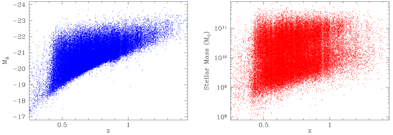
Fig. 13. The distribution of B -band luminosities (left) and stellar masses (right) computed for all objects with reliable redshift ( \text{flag} > 2.0 ) in the PDR-2 catalogue. These are estimated through SED fitting of all available photometry (from UV to K ) as described in Moutard et al. (2016b). Note that an explicit value of H_0 = 70 \text{ km s}^{-1} \text{ Mpc}^{-1} for the Hubble constant is used here.
