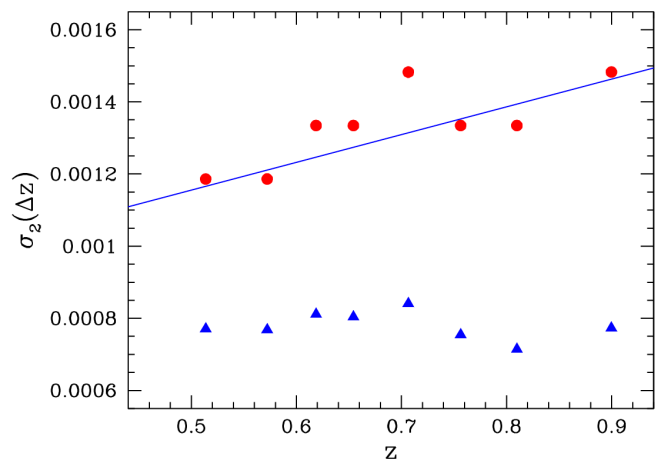
Fig. 11. The scatter in the \Delta z values (red circles) and in the \Delta z/(1+z) values (blue triangles) for objects in a narrow redshift bin, as a function of the median redshift for the bin. The bins are built to contain a fixed number of objects (500), and they are not statistically independent since they partly overlap each other. The blue line shows the mean scatter derived from the blue points, with the (1+z) scaling applied to it.
