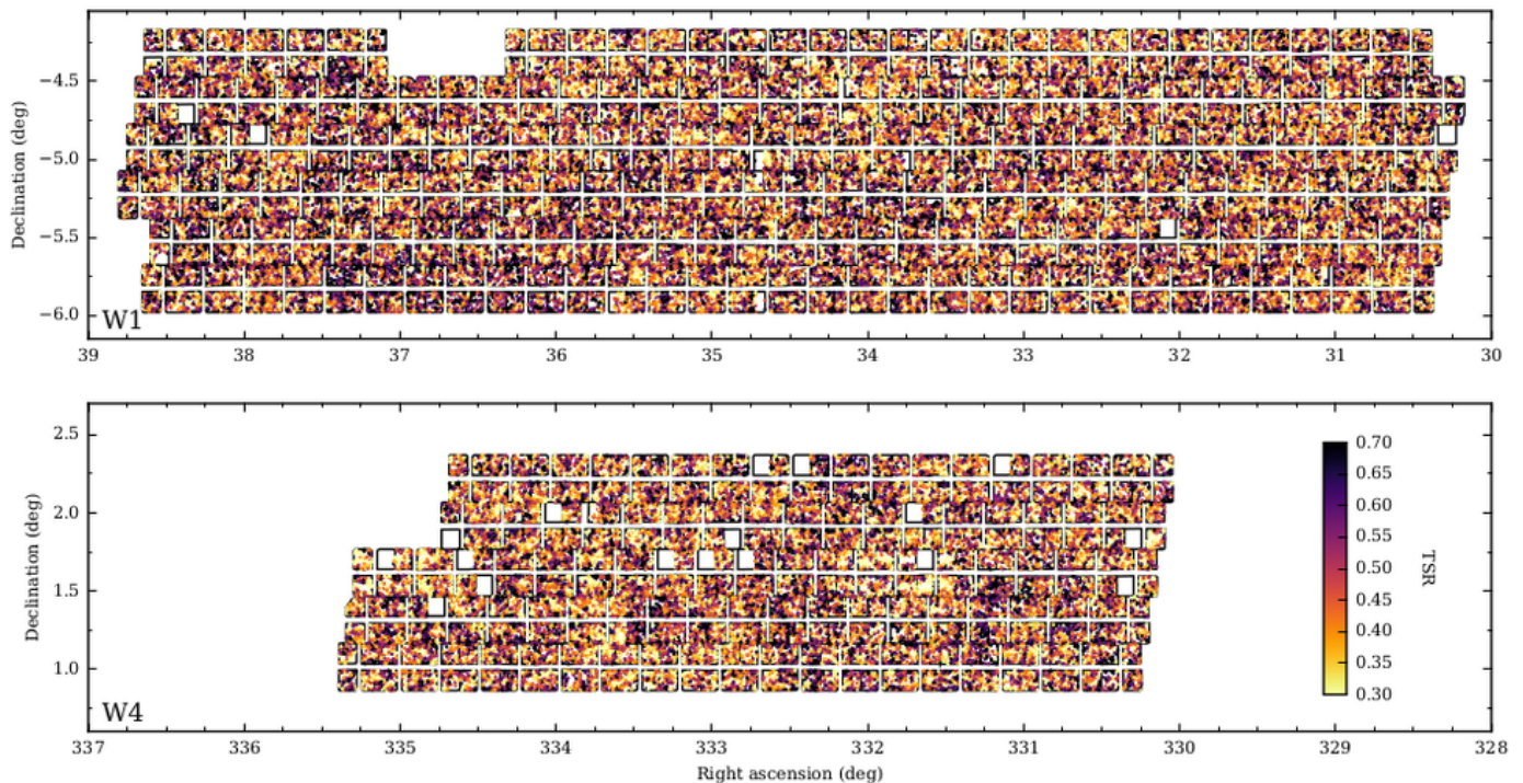
Fig. 5. The angular distribution over the survey areas of the Target Sampling Rate (TSR, colour scale), estimated locally for each galaxy as described in the text. In this plot, each value has been smoothed on a scale of 2 arcmin to enhance the (inverse) relationship of the TSR with the projected large-scale structure in the galaxy distribution.
