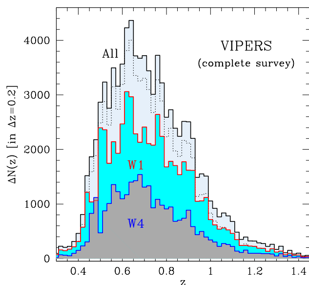
Fig. 12. The galaxy redshift distribution in the final VIPERS PDR-2 catalogue (black solid line), and separately within the W1 and W4 fields (red and blue solid lines, respectively). These include all measured redshifts, with flag 1 or larger. The dotted line shows the result of plotting only the flag \geq 2 galaxies, i.e. those that can be used reliably in statistical analyses.
