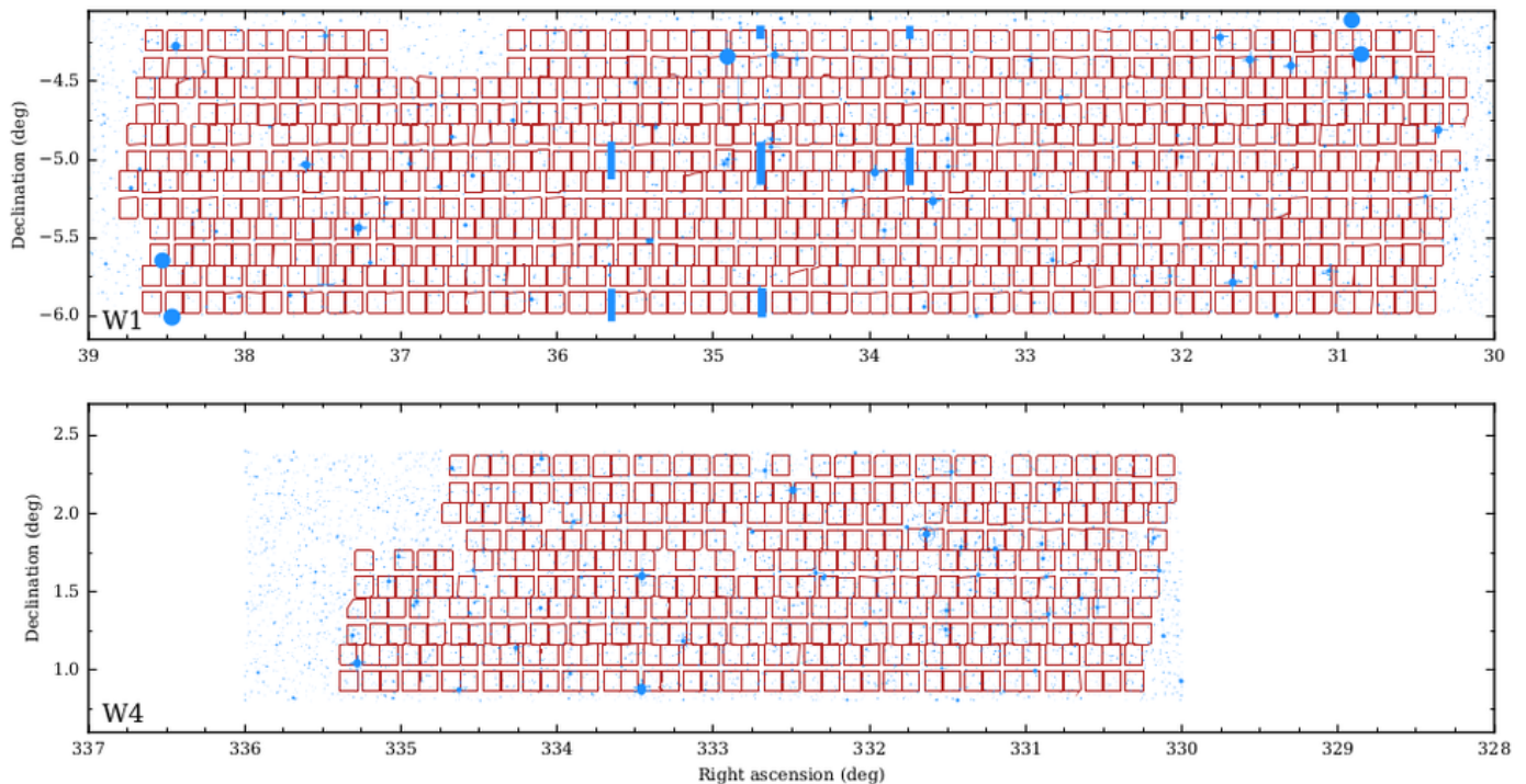
Fig. 2. The layout on the sky of all pointings that contribute to the PDR-2 final release, for the two fields W1 and W4, superimposed on the photometric survey mask. The contours of each of the four quadrants that comprise all VIMOS pointings are shown in red. The blue (grey) areas in the background correspond to areas where the parent photometry is corrupted or observations are not possible due to the presence of foreground objects, particularly bright stars and their diffraction spikes. Note that in this plot failed quadrants and other features introduced by the ‘spectroscopic mask’ are not indicated (see Section 3.2 and Figs 3 and 5).
