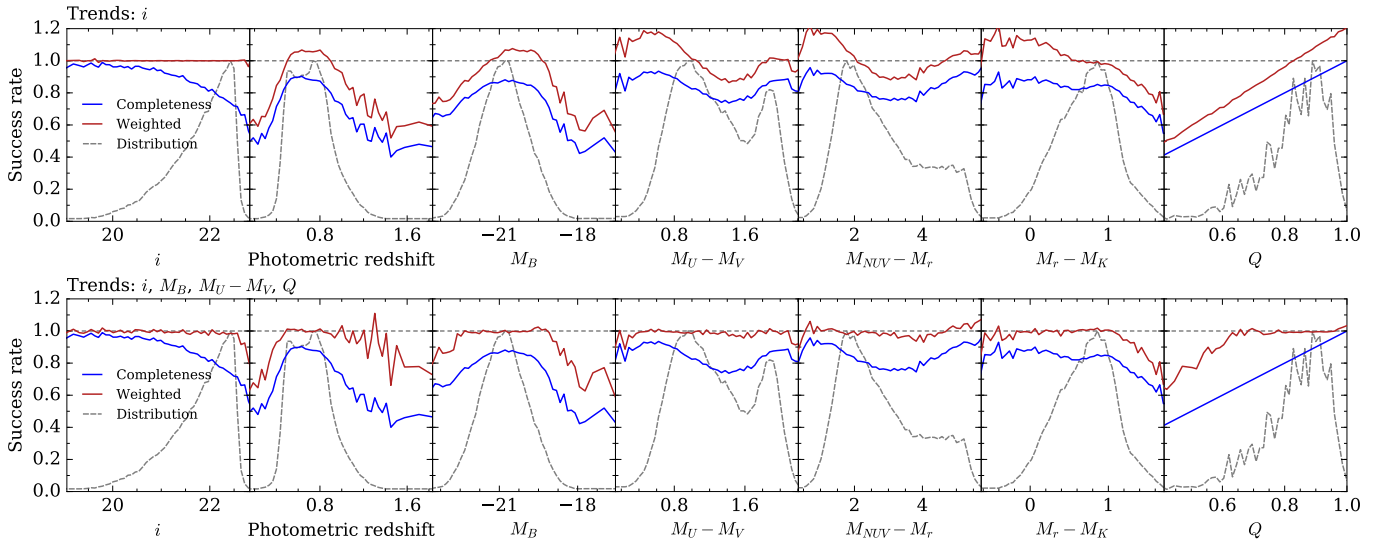
Fig. 6. The spectroscopic success rate (SSR) as a function of different observed photometric properties (blue solid curve), compared to the result of applying the weight to correct incompleteness (red solid curve). The two rows of plots show how the completeness correction changes when one only considers a simple SSR dependence on the selection i -band magnitude (top), or rather includes the more subtle dependencies on observed colours and, in particular, quality of the specific VIMOS quadrant ( Q parameter, quantified via the mean SSR for all galaxies in that quadrant). The differential distribution of each parameter is also plotted in each panel (dashed curve).
