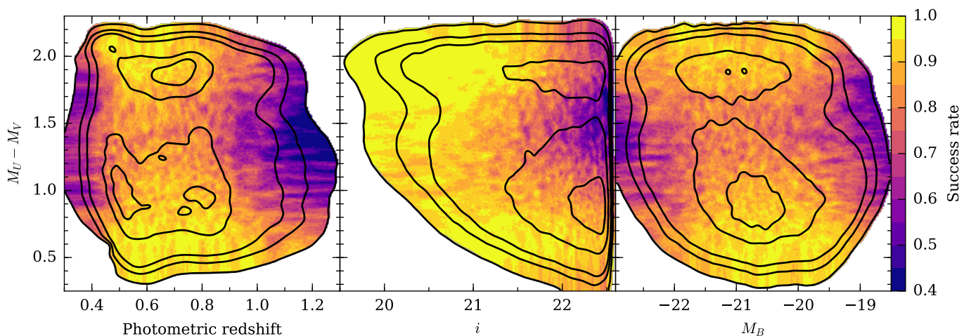
Fig. 7. 2D plots of the SSR in the photometric parameter space. We show the dependence on the rest-frame U - V colour jointly with three photometric parameters: photometric redshift (left), apparent i -band magnitude (centre), and rest-frame B -band magnitude (right). The solid contours contain 10, 50, 90 and 99% of the sample.
