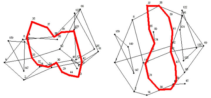
Fig. 2. Deflection shape of tested motor at f_s(38/2 + 4) = 23f_s , with f_s = 30 Hz (no load case), captured at two successive moments.
