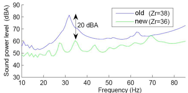
Fig. 6. Sound power level radiated by initial tested motor with Z_r = 38 , where a strong saturation vibration resonates with stator elliptical mode, and by proposed motor with a 36 slots rotor.
