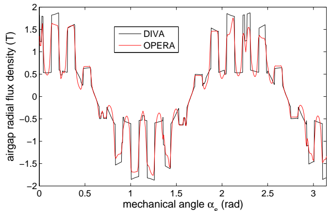
Fig. 5. FEM and DIVA flux density distribution along the air-gap in saturated case.
