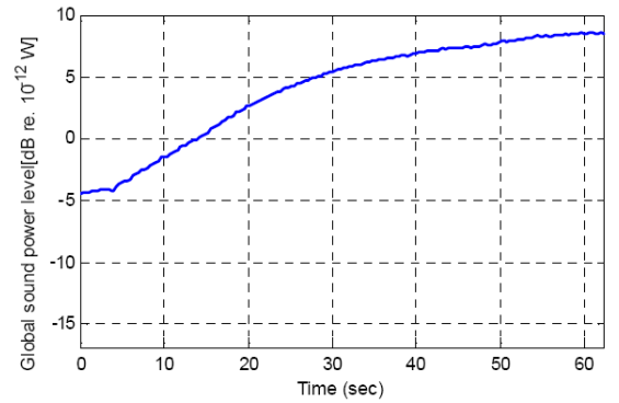
Fig. 3. Normalized evolution of sound power level due to saturation with time, when linearly increasing the air-gap flux from 2 to 7.5 V/Hz.
