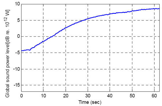
Fig. 3. Normalized evolution of sound power level due to saturation with time, when linearly increasing the air-gap flux from 2 to 7.5 V/Hz.
