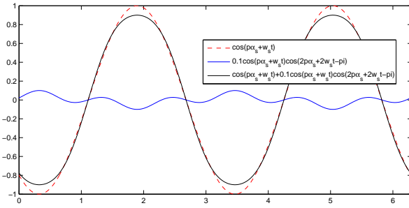
Fig. 1. Illustration of the air-gap radial flux density flattening due to even order saturation permeance waves.
