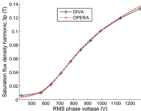
Fig. 4. FEM and DIVA main flux density saturation harmonic of spatial order 3p in function of the applied phase voltage, after having fit the analytical model.
