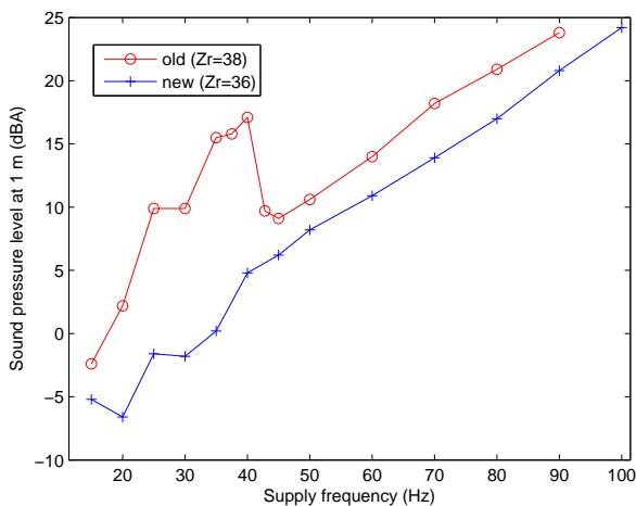
Fig. 7. Sound pressure level radiated by initial motor with Z_r = 38 , where a strong saturation vibration resonates with stator elliptical mode, and by the proposed new motor with 36 rotor slots. A normalization factor has been introduced for confidentiality reasons.
