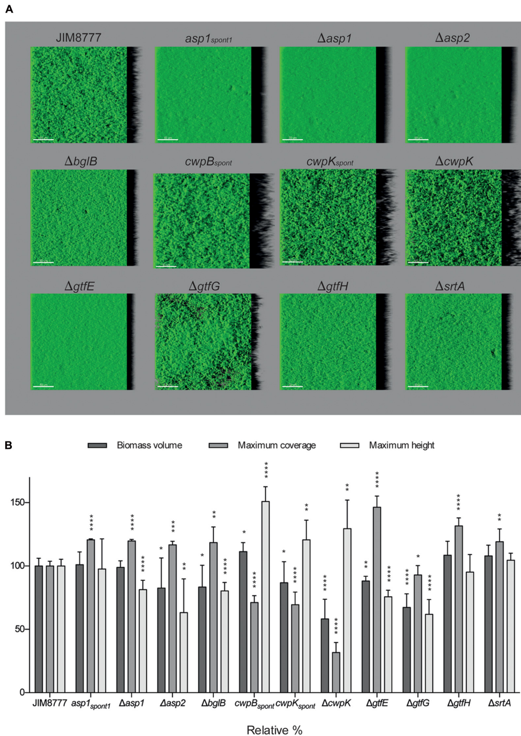
FIGURE 3 | Auto-aggregation factors of JIM8777 and their impact on biofilm architecture. (A) 3-D reconstructions of representative confocal images of 5-h-old biofilms formed by S. salivarius strains. Scale bars: 50 \mu\text{m} . (B) Biomass volume ( \mu\text{m}^3 ), maximum coverage (%) and maximum height ( \mu\text{m} ) were normalized against values obtained for JIM8777 and measured for each strain in nine different CLSM image stacks from two independent experiments. Student's t -test was used for statistical analysis (**** P < 0.0001 , *** P < 0.0005 , ** P < 0.005 , * P < 0.05 ).
